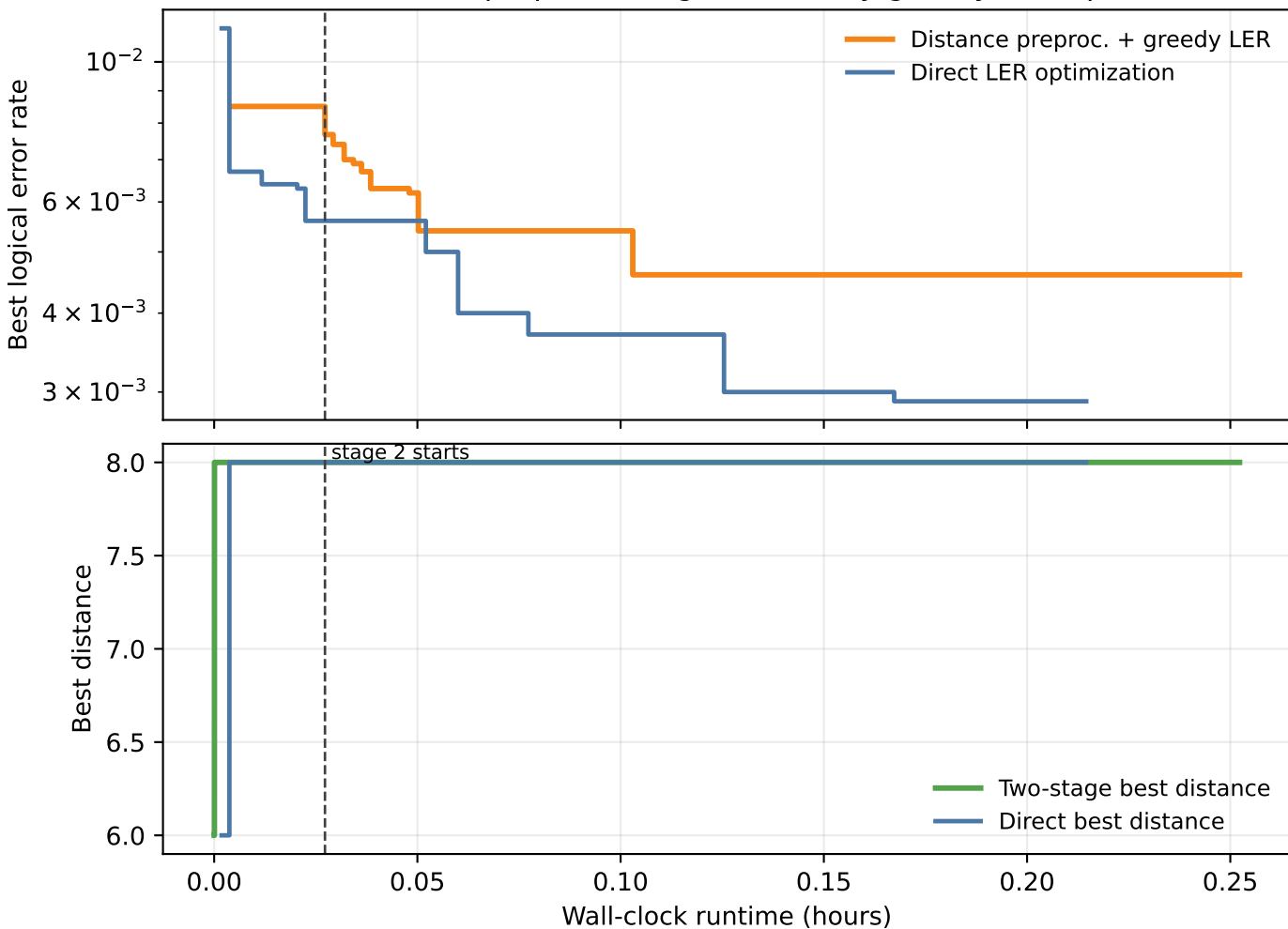
[625,25]: distance preprocessing followed by greedy LER optimization
