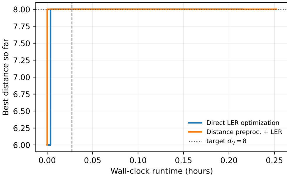
[625,25]: time to target distance
