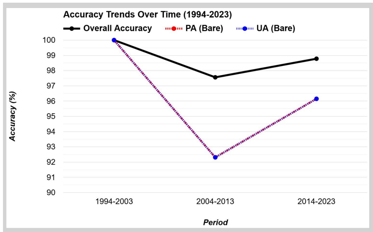
Figure 5-2: Model Accuracy
