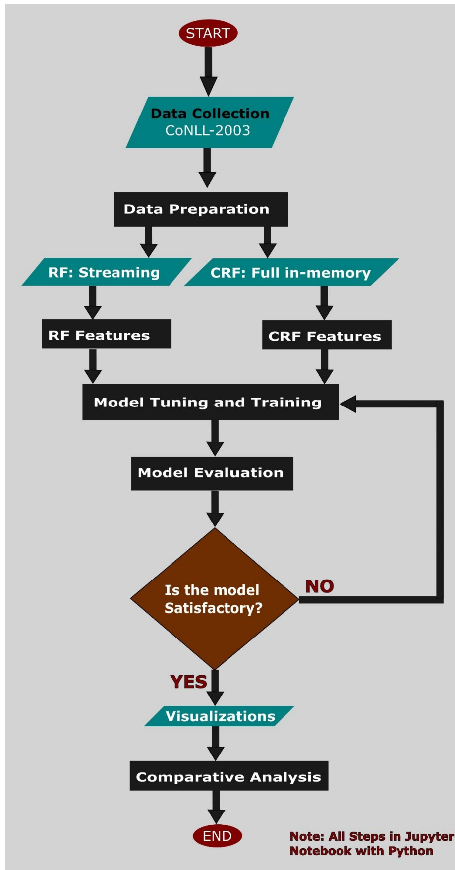
Figure 3-1: Implementation Flowchart
