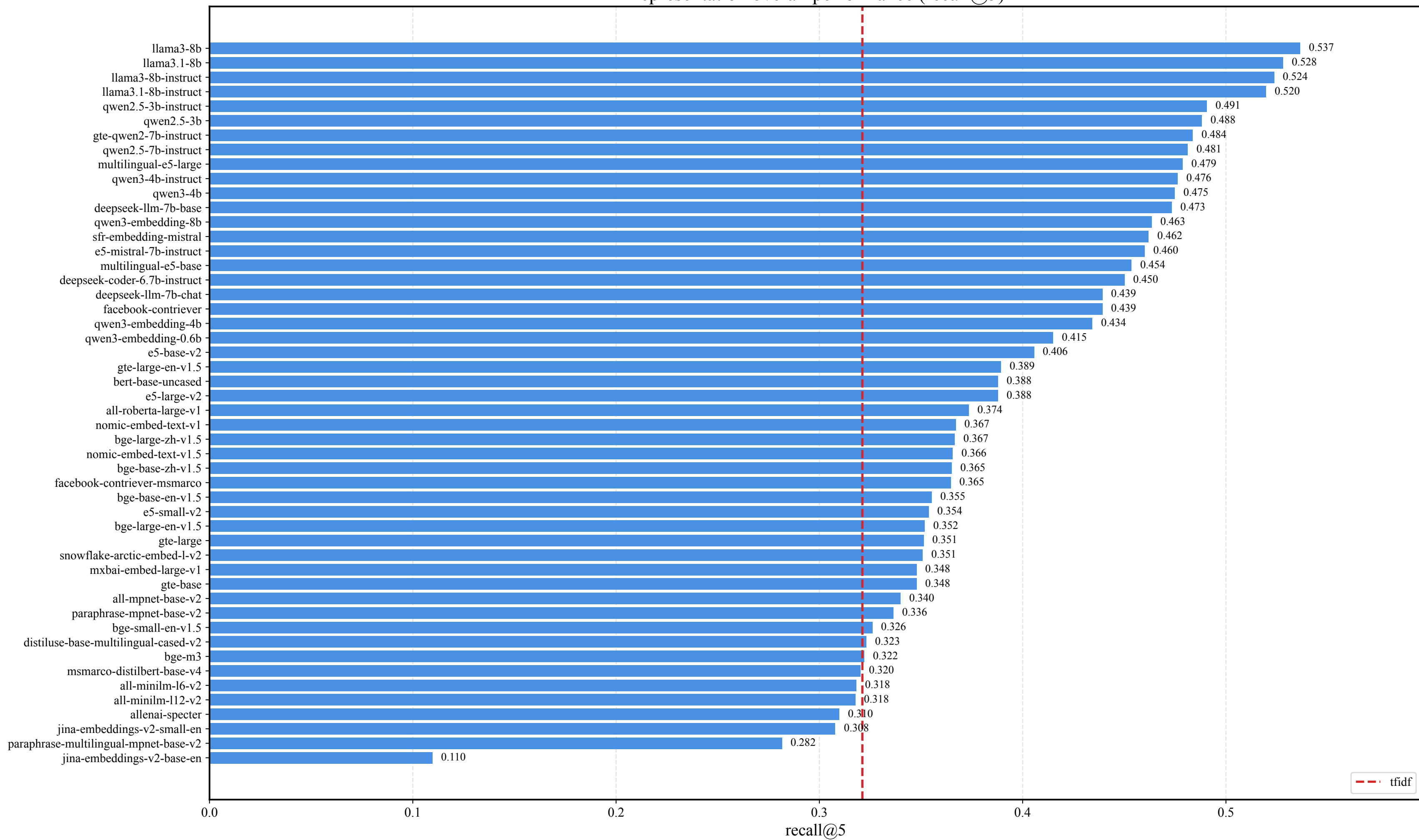
Representation overall performance (recall@5)
