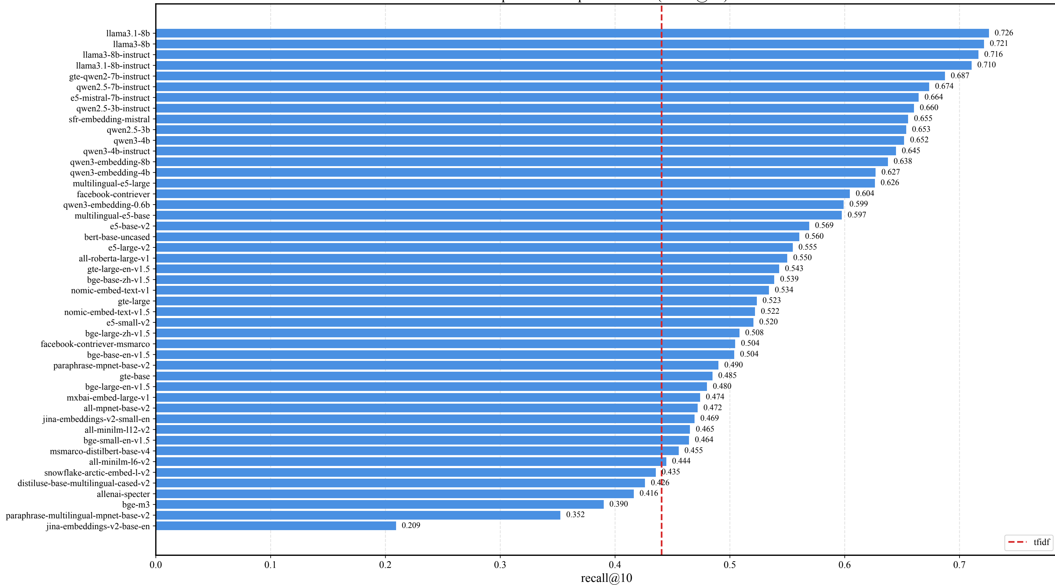
Representation performance (recall@10)
