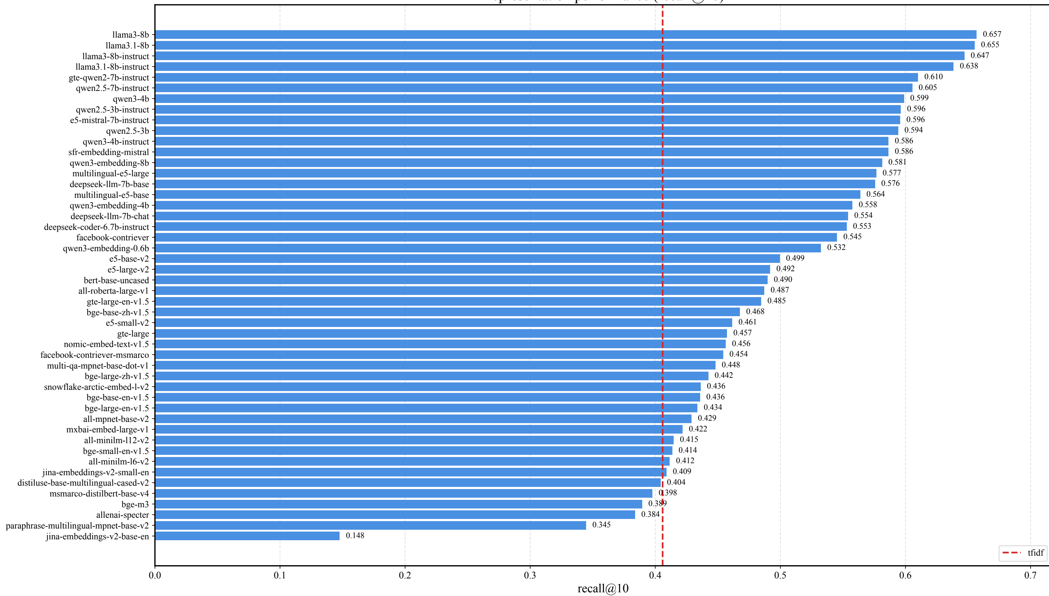
Representation performance (recall@10)
