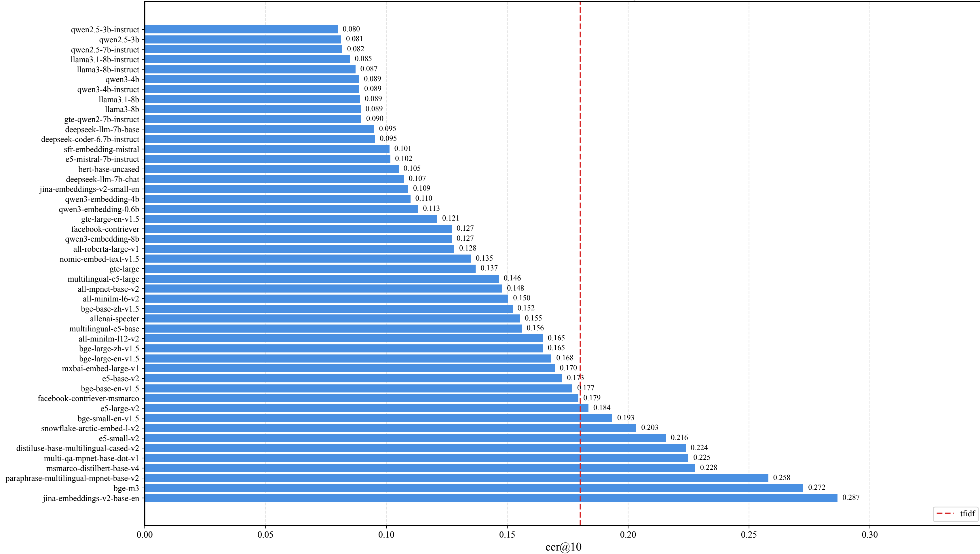
Attribution performance (eer@10)
