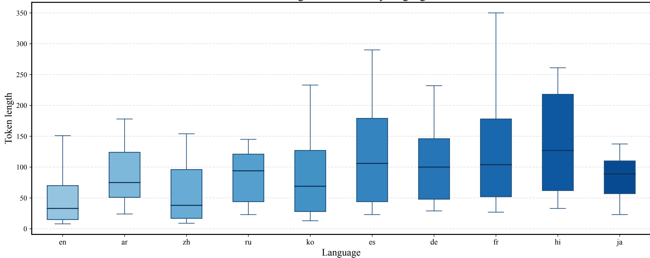
Token length distribution by language
