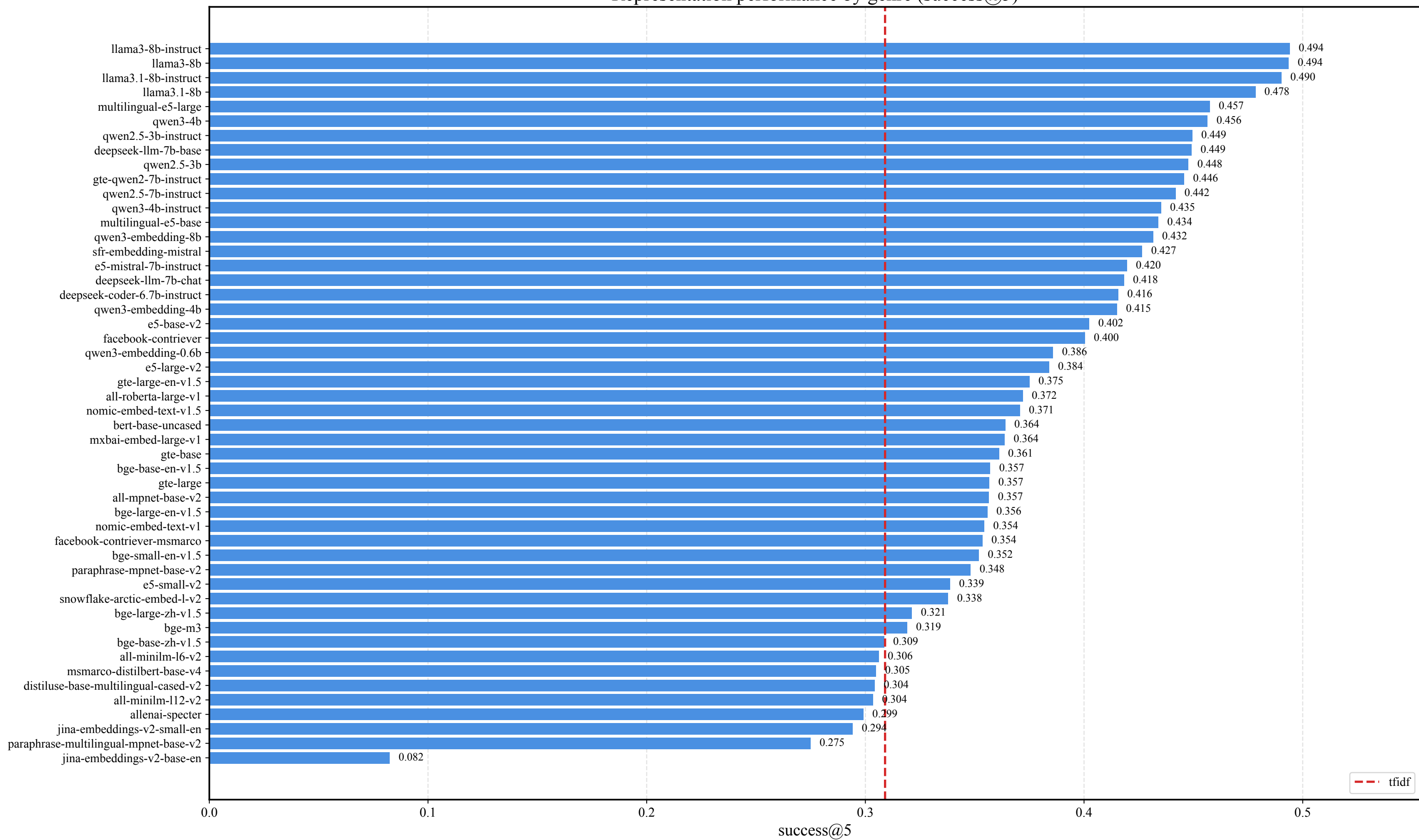
Representation performance by genre (success@5)
