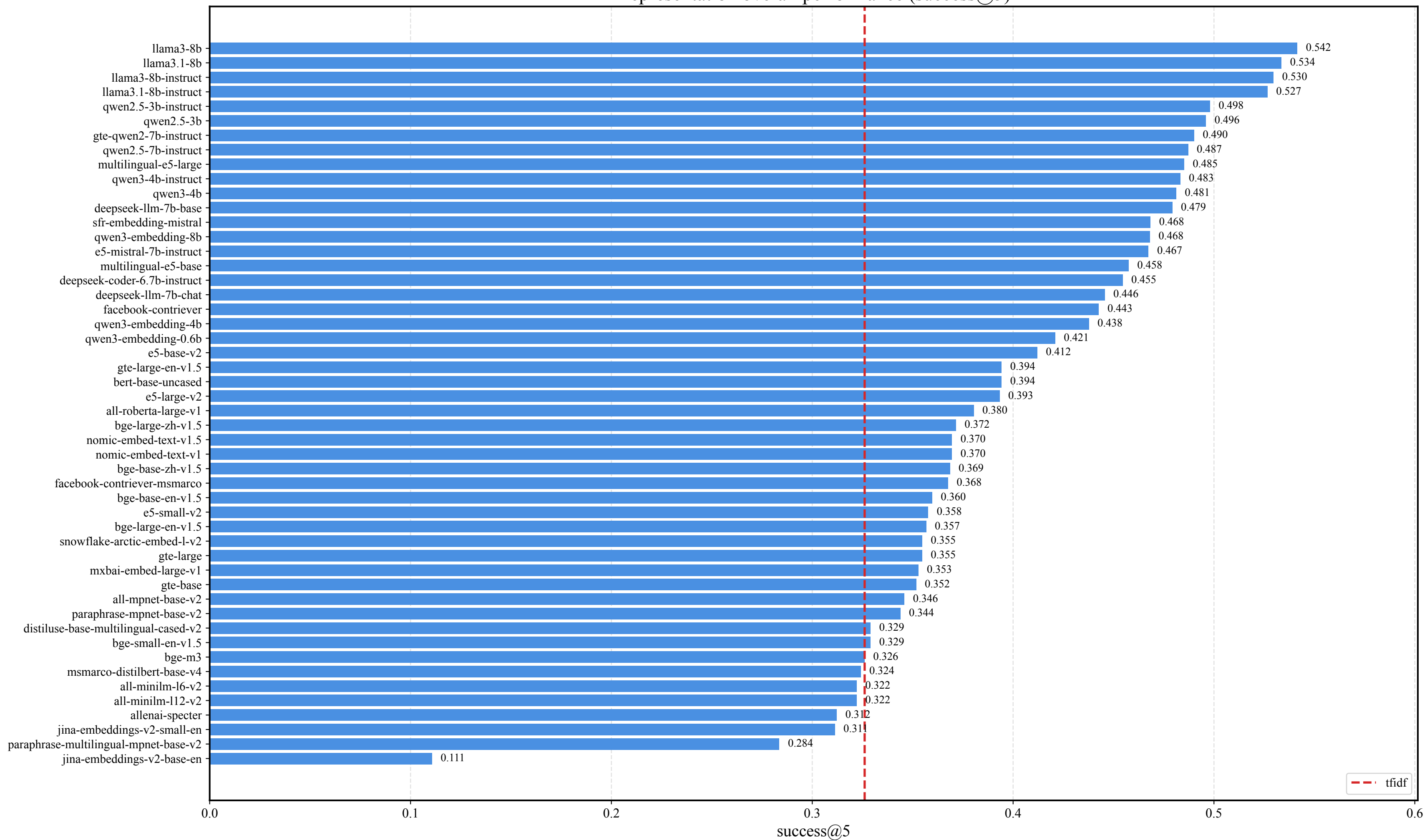
Representation overall performance (success@5)
