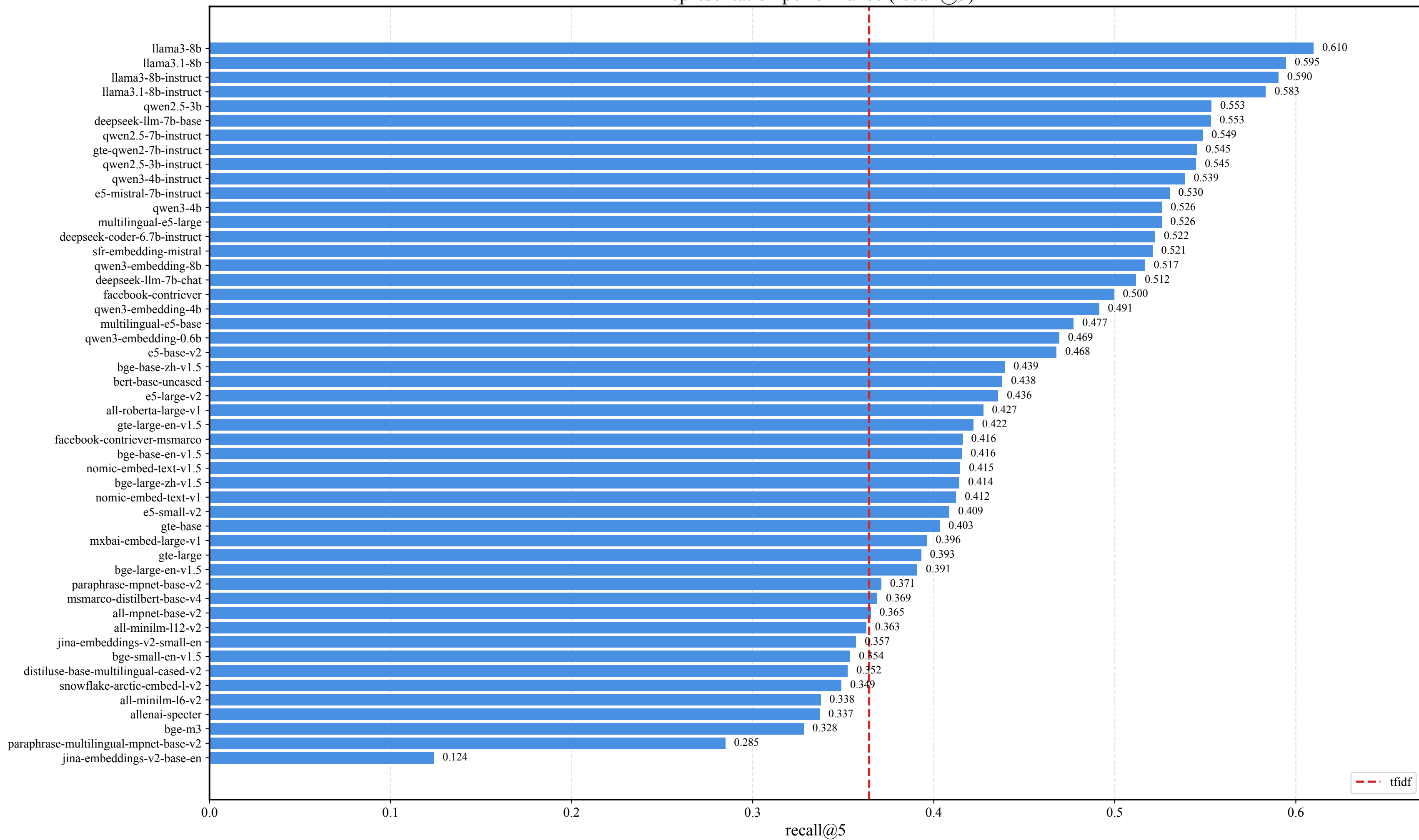
Representation performance (recall@5)
