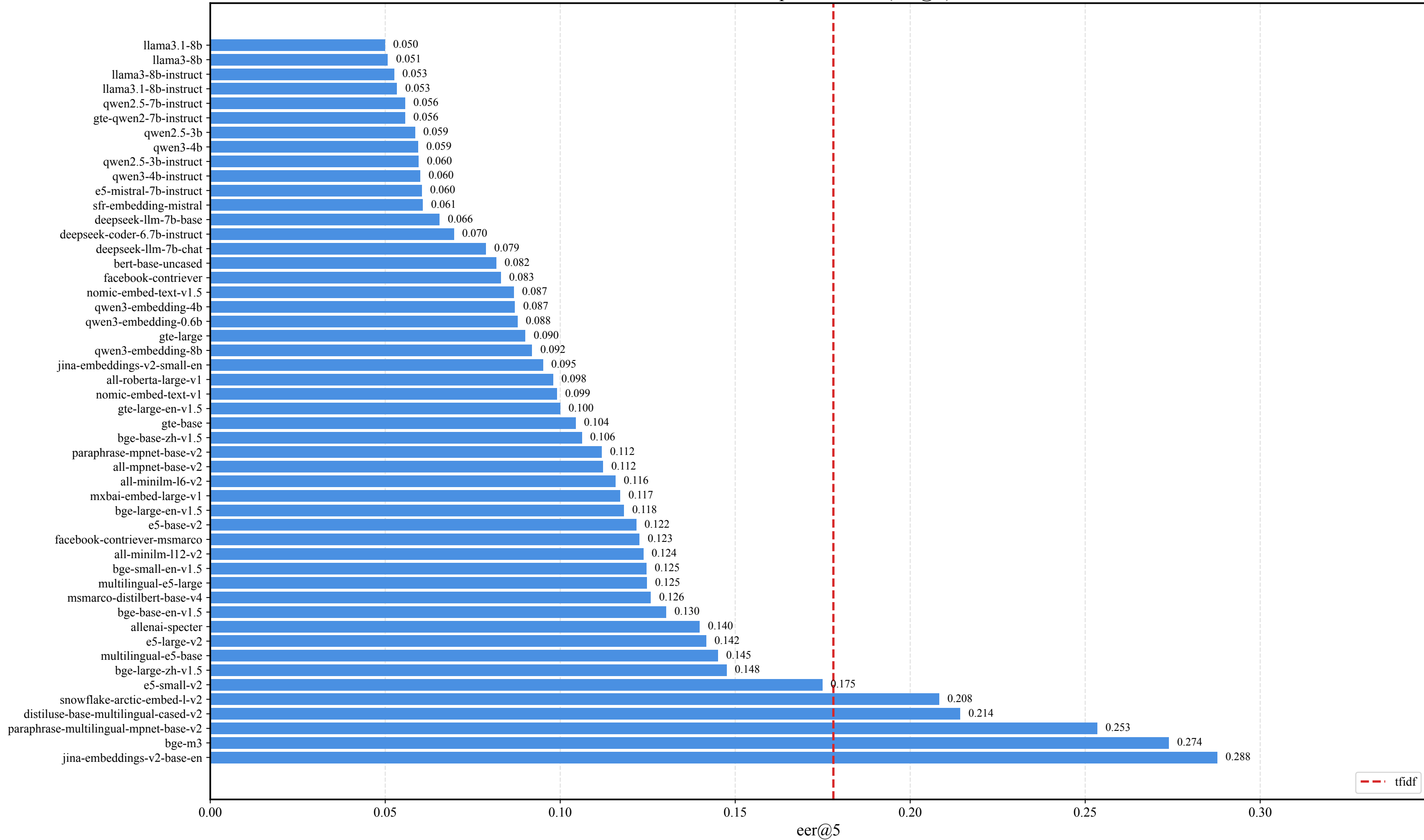
Attribution performance (eer@5)
