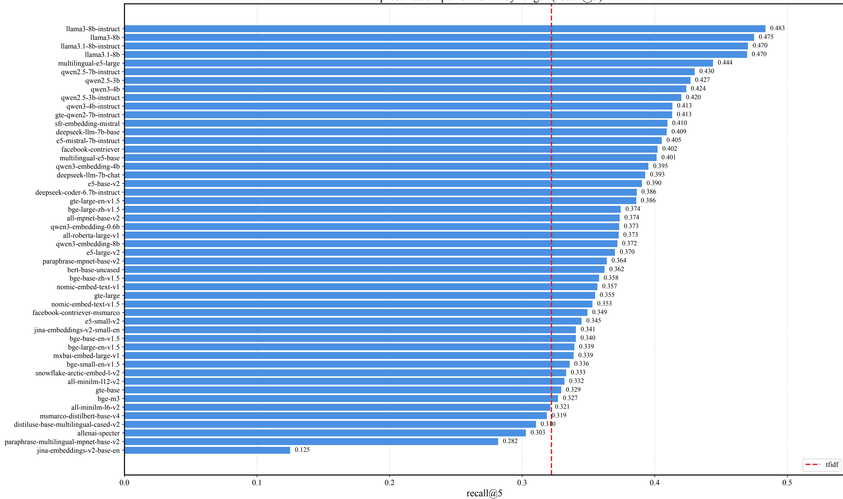
Representation performance by length (recall@5)
