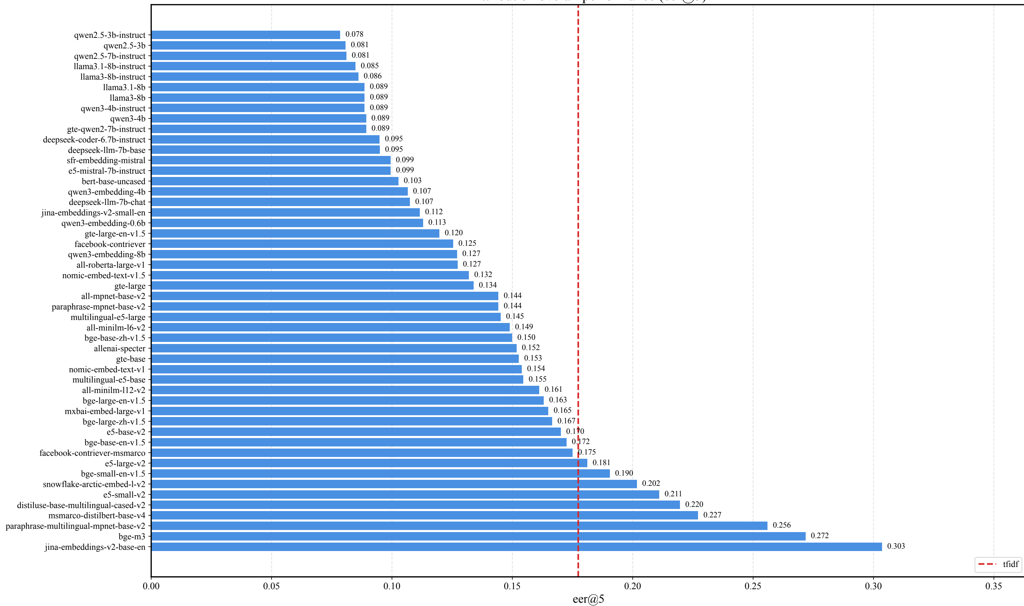
Attribution overall performance (eer@5)
