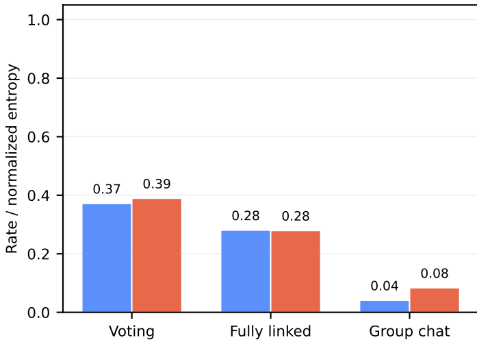
Mean normalized entropy
