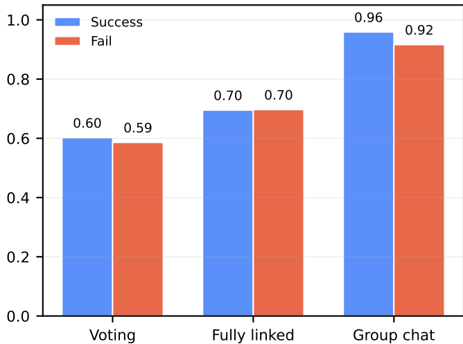
Single-option tally rate
