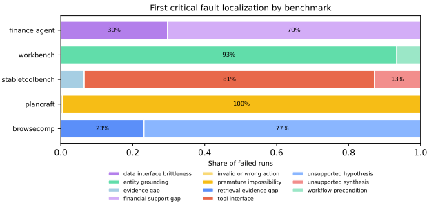
Figure 7. First critical fault localization over failed runs. The earliest visible bottleneck is benchmark-specific, supporting the claim that topology operates on top of benchmark-anchored failure regimes.
