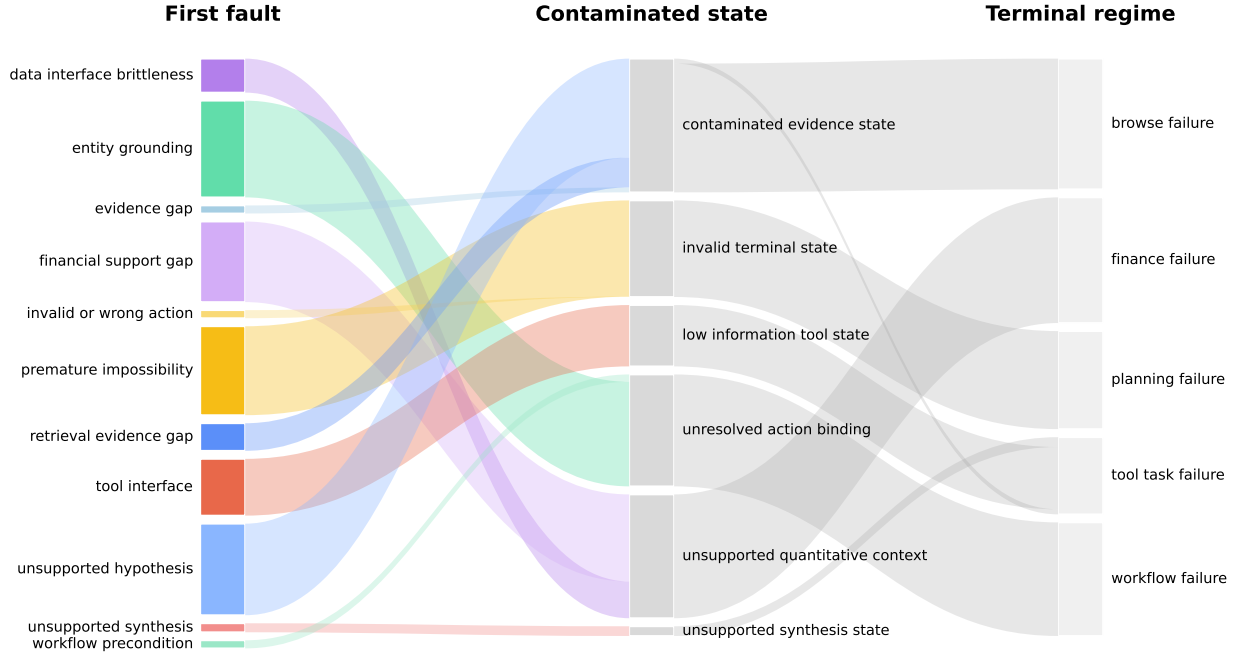
Figure 8. Aggregate diagnostic flow from first critical fault to contaminated state and terminal failure regime. The flow should be read as heuristic localization over traces, not as a formal causal graph.
