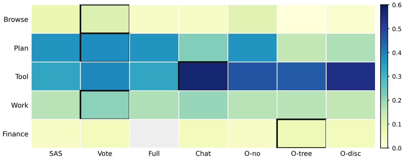
Task success by topology
