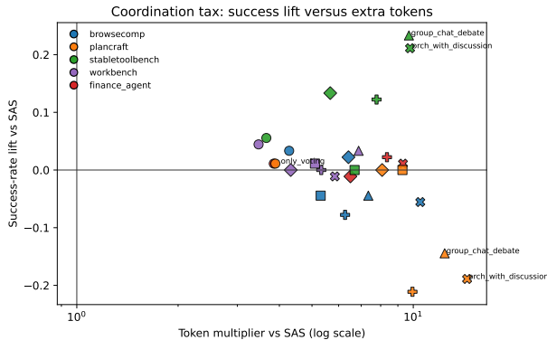
Figure 6. Coordination tax: success lift versus token multiplier relative to the single-agent baseline. StableToolBench is the only clear high-cost, high-gain case.
