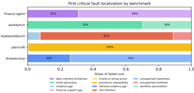
Figure 8. First critical fault localization over failed runs. The earliest visible bottleneck is benchmark-specific, supporting the claim that topology operates on top of benchmark-anchored failure regimes.
