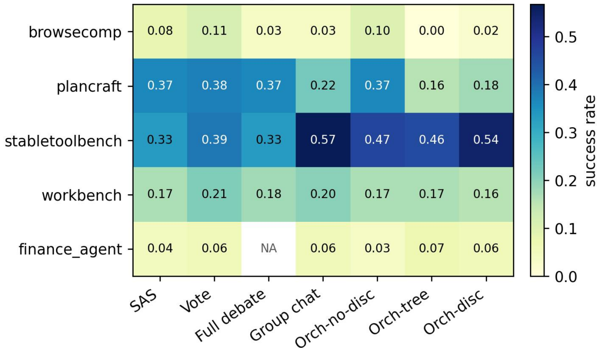
Task success by benchmark and topology
