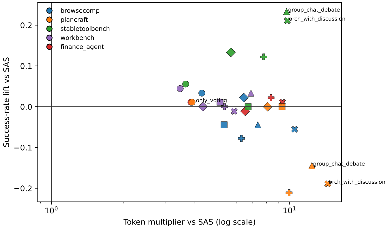
Coordination tax: success lift versus extra tokens
