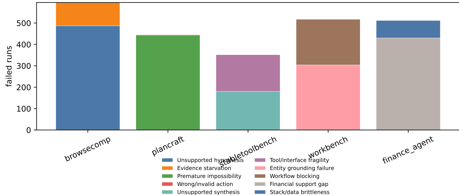
Failure regimes aggregated across topology slices
