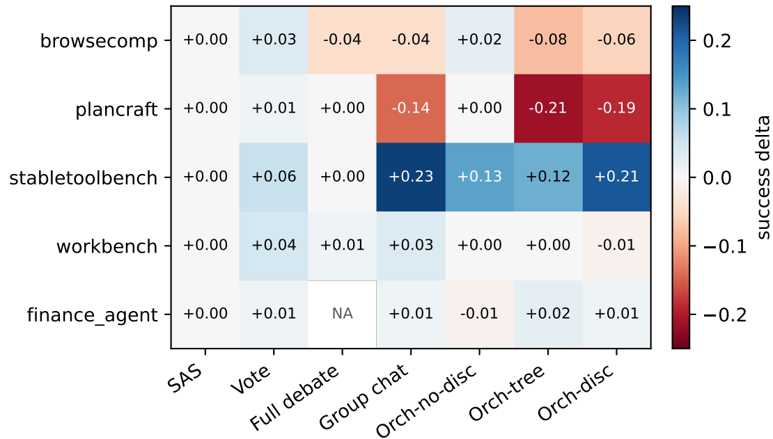
Success lift relative to SAS
