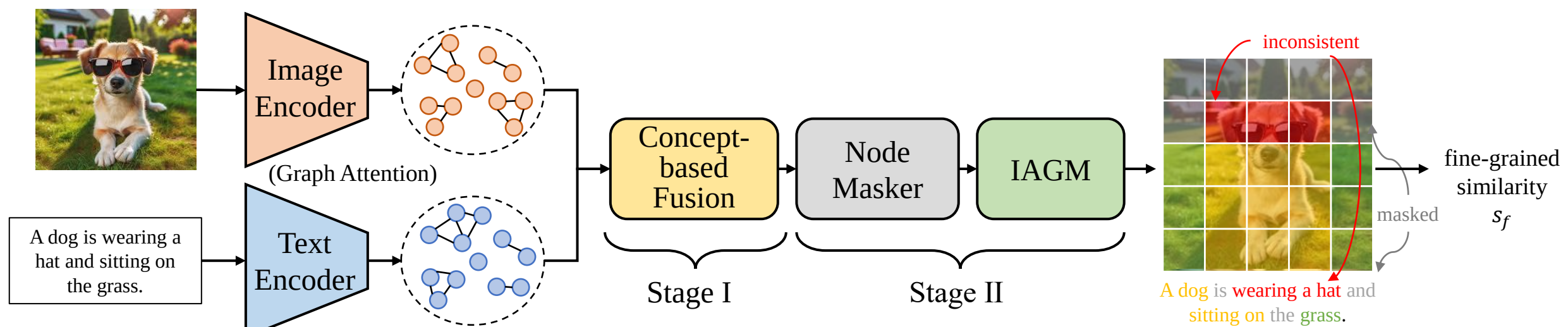
(a) Graph learning-based fine-grained multimodal alignment method GFGA
