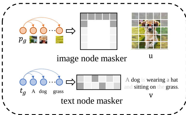
(c) Node masker
