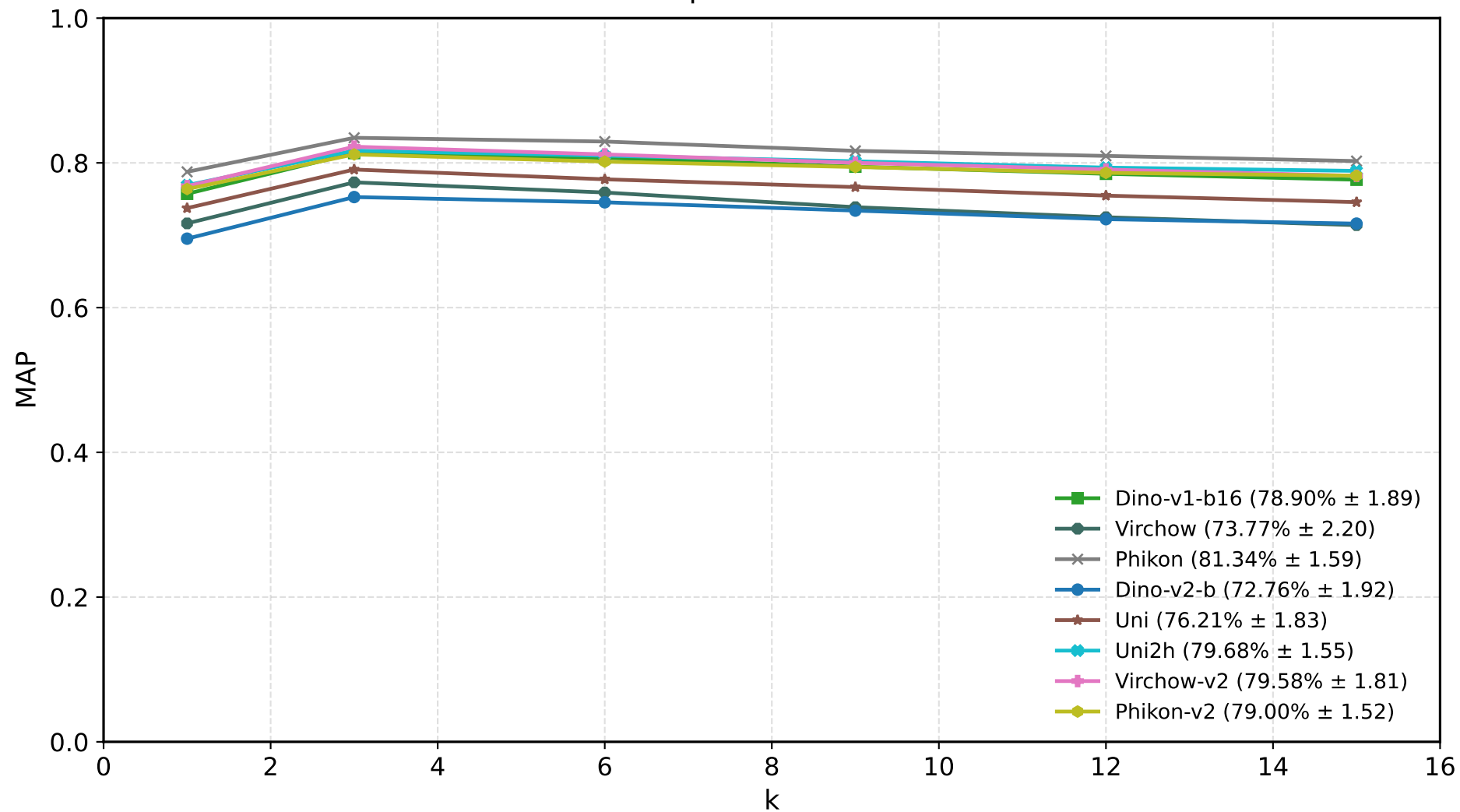
Model Comparison on Glomerulus
