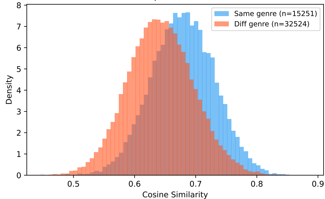
LLM Profile (bge-large-v1.5, 1024d)
