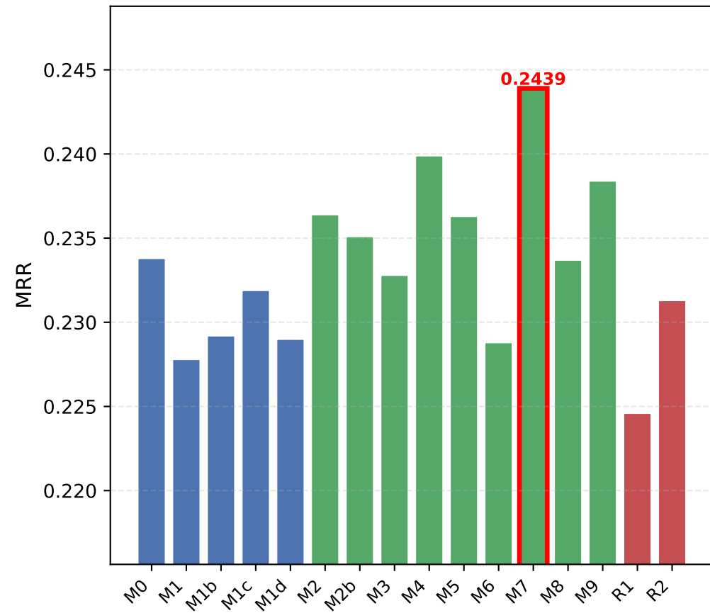
MRR (higher is better)
