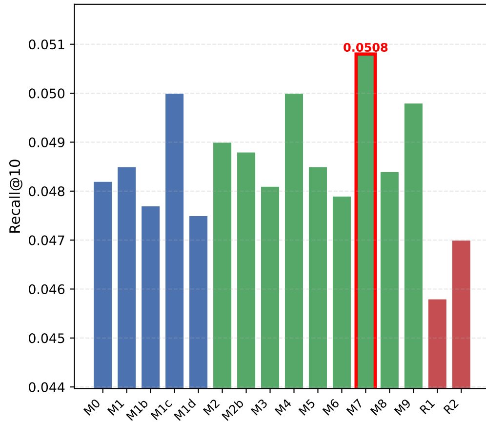
Recall@10 (higher is better)
