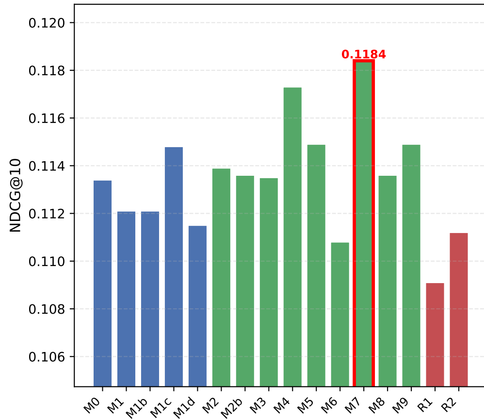
NDCG@10 (higher is better)
