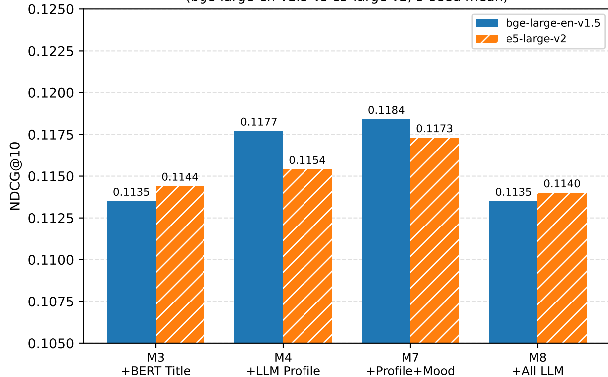
Encoder Sensitivity (bge-large-en-v1.5 vs e5-large-v2, 5-seed mean)
