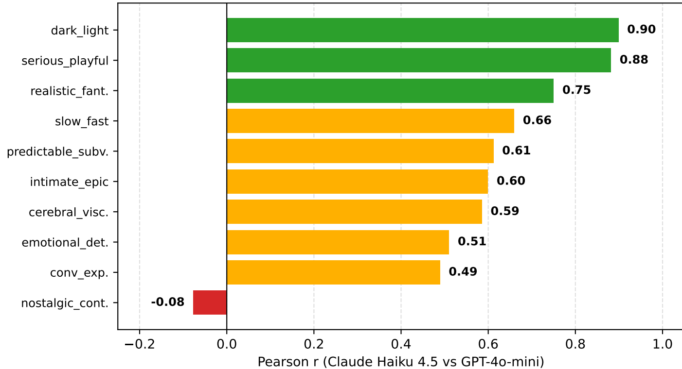
LLM Sensitivity: Mood Vector Correlation (500 profiles, identical prompt)
