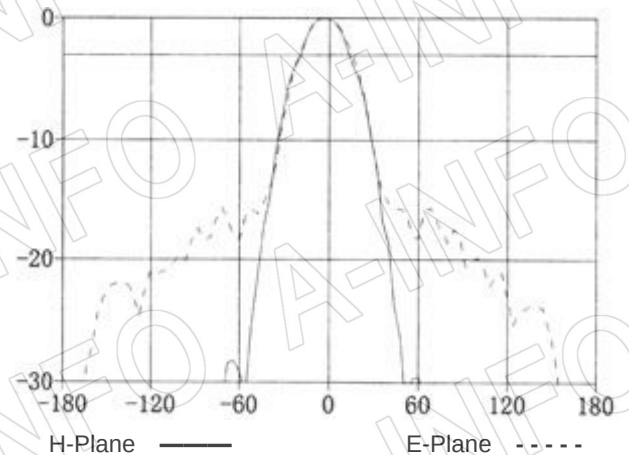
Frequency: 18.0GHz
