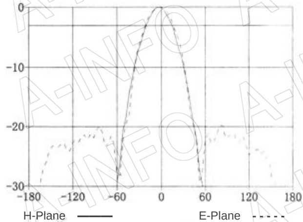
Frequency: 16.5GHz
