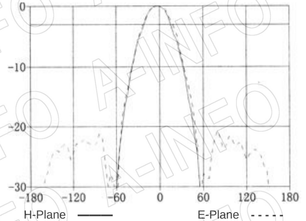
Frequency: 16.0GHz
