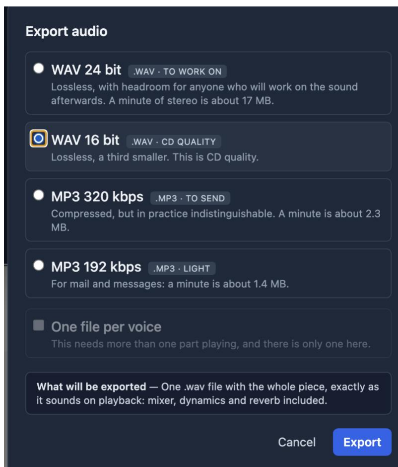
Figure — The audio export window: the format, the tick for separate voices and the summary of what will be written.
