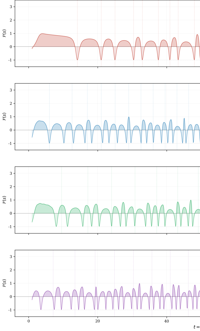
FIG. 8: Interference fingerprints \mathcal{F}(\frac{1}{2} + it) for four L -functions. Dashed vertical lines mark the first non-trivial zeros of each function; at every zero, \mathcal{F} \approx -1 (complete destructive interference). Each L -function exhibits a distinctive interference pattern that serves as its arithmetic “fingerprint.” Shaded regions indicate constructive ( \mathcal{F} > 0 , lighter) and destructive ( \mathcal{F} < 0 , darker) interference.
