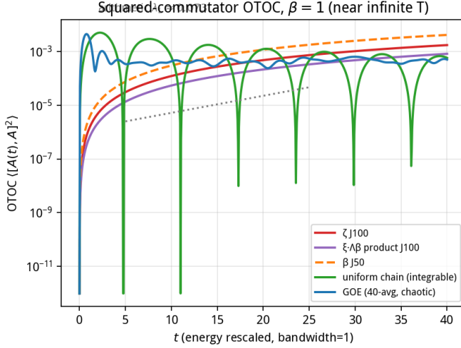
FIG. 7: Out-of-time-order correlator C(t) (log scale). Left: \beta = 1 comparison of five systems: GOE ensemble (40 realizations, instantaneous scrambling), arithmetic chains ( \zeta -J100, \beta -J50, product-J100, all smooth monotonic growth, \lambda_L \approx 0.073 ), uniform chain (periodic revivals, integrable). Right: \zeta -J100 at five inverse temperatures \beta = 0.5, 1, 2, 5, 10 ; the curves overlap, showing \lambda_L is temperature-independent.
