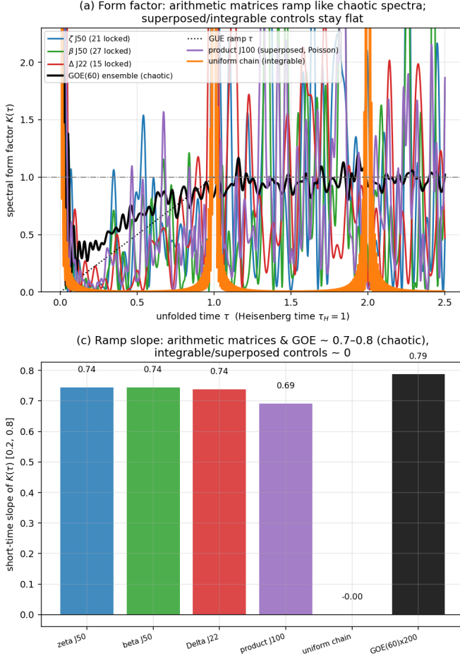
FIG. 2: Experiment 2. (a) Spectral form factor: the three arithmetic Hamiltonians ramp with slope \approx 0.74 like the GOE ensemble (0.79); the uniform chain is flat. (b) Survival: the integrable chain revives perfectly at \tau_H ( P = 0.993 ); arithmetic and GOE spectra decay aperiodically with no revival. (c) Ramp-slope summary. (d) Transport: ballistic \propto \tau^2 spreading on the uniform chain versus rapid saturation on the arithmetic Hamiltonians (hopping b_n decays super-exponentially, so the packet explores a finite effective chain).
