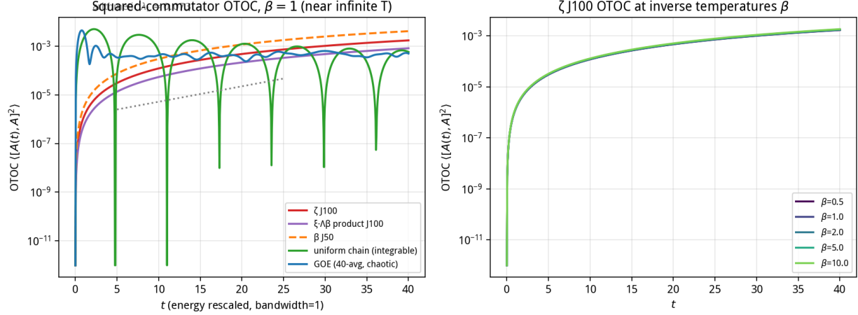
Figure 4: Out-of-time-order correlator C(t) (log scale). Left: \beta = 1 comparison of five systems: GOE ensemble (40 realizations, instantaneous scrambling), arithmetic chains ( \zeta -J100, \beta -J50, product-J100, all smooth monotonic growth, \lambda_L \approx 0.073 ), uniform chain (periodic revivals, integrable). Right: \zeta -J100 at five inverse temperatures \beta = 0.5, 1, 2, 5, 10 ; the curves overlap, showing \lambda_L is temperature-independent.
