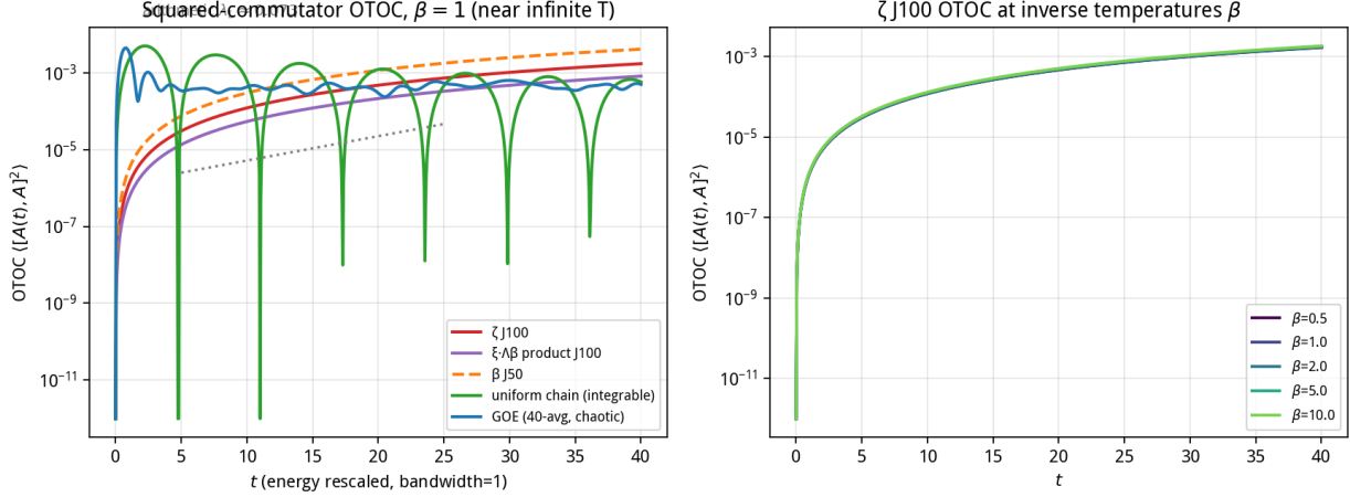
Figure 7: Out-of-time-order correlator C(t) (log scale). Left: \beta = 1 comparison of five systems: GOE ensemble (40 realizations, instantaneous scrambling), arithmetic chains ( \zeta - J100 , \beta - J50 , product- J100 , all smooth monotonic growth, \lambda_L \approx 0.073 ), uniform chain (periodic revivals, integrable). Right: \zeta - J100 at five inverse temperatures \beta = 0.5, 1, 2, 5, 10 ; the curves overlap, showing \lambda_L is temperature-independent.
