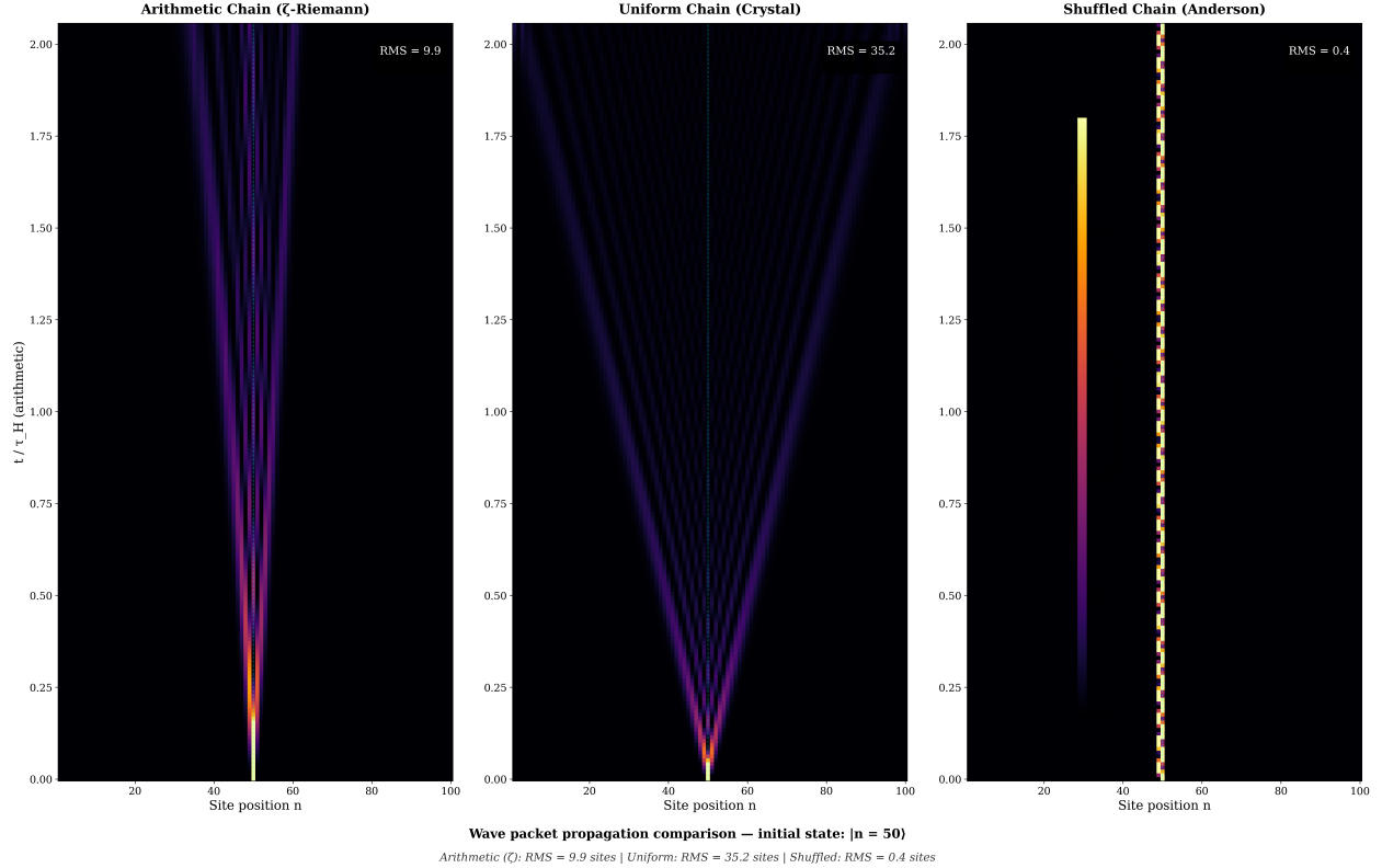
Figure 3: Experiment 2 (Supplementary). Spatiotemporal evolution |\langle n | \psi(t) \rangle|^2 of a wave packet initialized at the chain center |n=50\rangle for three chains sharing identical coefficient distributions. Left: arithmetic \zeta -Jacobi chain — restricted spreading with RMS displacement \approx 10 , neither ballistic nor fully localized (“pseudo-Anderson” behavior). Center: uniform crystal chain — ballistic light-cone spreading, \text{RMS} \approx 35 . Right: shuffled Anderson chain — complete localization, \text{RMS} \approx 0.4 ; the wave packet is frozen at the initial site.
