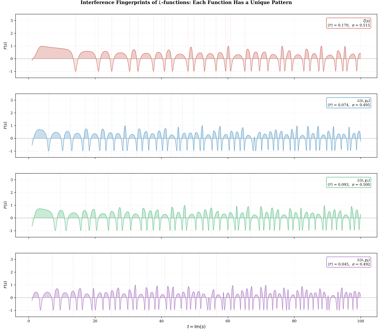
Figure 8: Interference fingerprints \mathcal{F}(\frac{1}{2}+it) for four L -functions. Dashed vertical lines mark the first non-trivial zeros of each function; at every zero, \mathcal{F} \approx -1 (complete destructive interference). Each L -function exhibits a distinctive interference pattern that serves as its arithmetic “fingerprint.” Shaded regions indicate constructive ( \mathcal{F} > 0 , lighter) and destructive ( \mathcal{F} < 0 , darker) interference.
