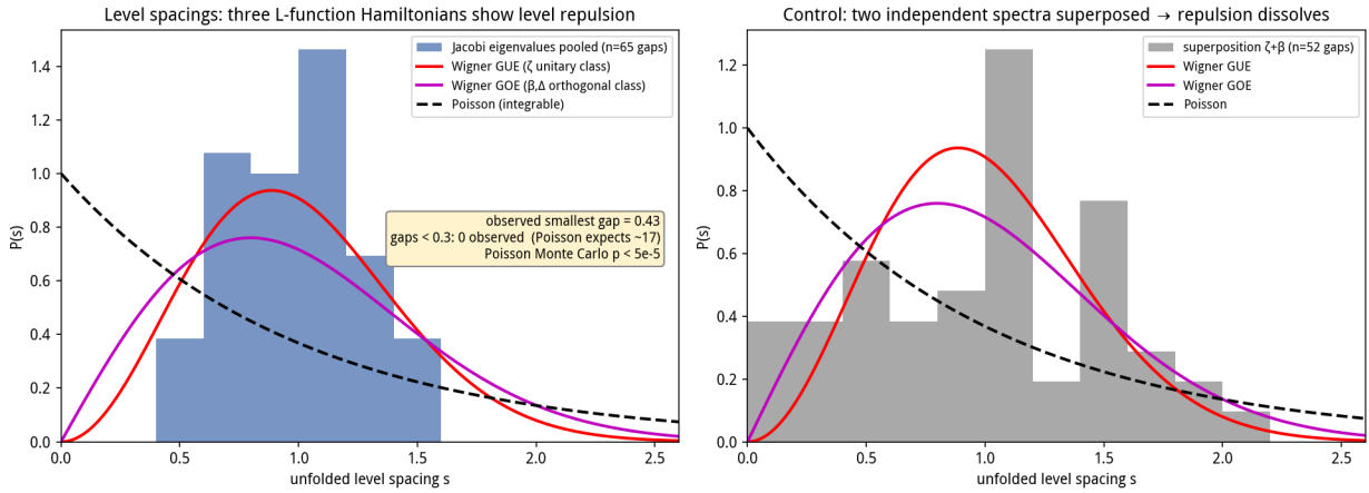
Figure 1: Experiment 1. Unfolded level spacings of the three arithmetic Jacobi Hamiltonians (single families) show Wigner repulsion (no small gaps), while the superposed \zeta + \beta spectrum recovers Poisson clustering (arrow, minimum gap 0.044).
