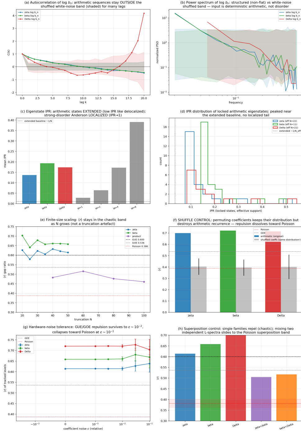
FIG. 7: Experiment 3 evidence chain. (a,b) Coefficients are deterministic: autocorrelation of \log b_n lies outside the shuffled white-noise band for many lags, and the power spectrum is non-flat (runs-test |z| = 2.9\text{--}6.6 ). (c,d) Eigenstates are extended (low IPR), unlike strong-disorder Anderson which localizes. (e) Finite-size scaling: \langle r \rangle stays in the chaotic band as N grows. (f) SHUFFLE CONTROL : permuting \alpha_n, b_n keeps their distribution but destroys the recurrence, and \langle r \rangle collapses to Poisson while IPR rises to localized values. (g) Robustness to multiplicative coefficient noise up to \sim 10\% . (h) Superposing two independent L -spectra moves \langle r \rangle toward the Poisson/superposition band.
