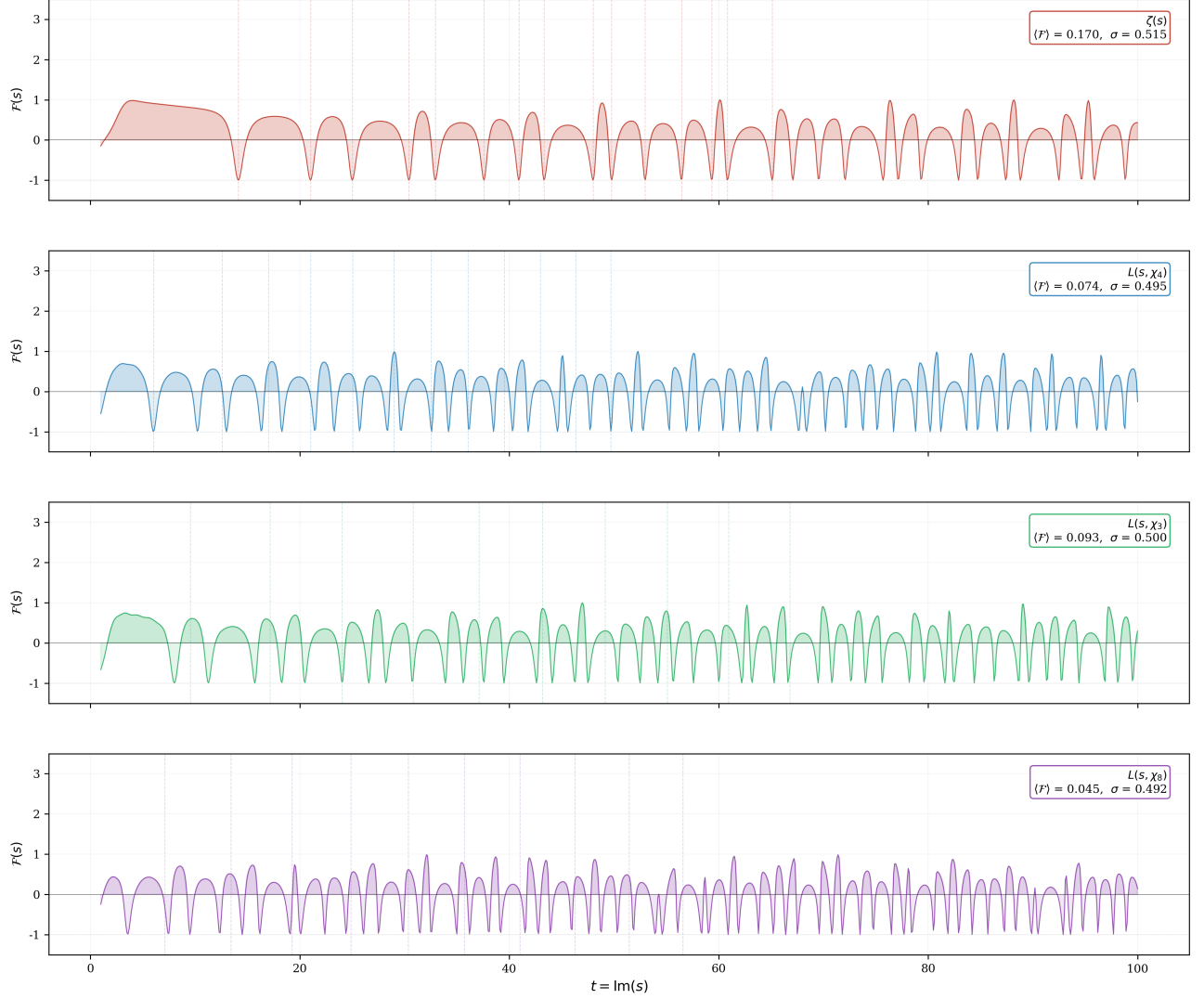
FIG. 9: Interference fingerprints \mathcal{F}(\frac{1}{2} + it) for four L -functions. Dashed vertical lines mark the first non-trivial zeros of each function; at every zero, \mathcal{F} \approx -1 (complete destructive interference). Each L -function exhibits a distinctive interference pattern that serves as its arithmetic “fingerprint.” Shaded regions indicate constructive ( \mathcal{F} > 0 , lighter) and destructive ( \mathcal{F} < 0 , darker) interference.
