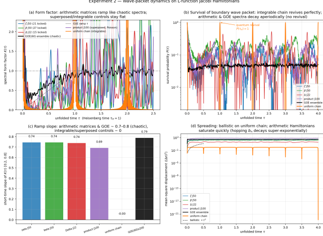
FIG. 3: Experiment 2. (a) Spectral form factor: the three arithmetic Hamiltonians ramp with slope \approx 0.74 like the GOE ensemble (0.79); the uniform chain is flat. (b) Survival: the integrable chain revives perfectly at \tau_H ( P = 0.993 ); arithmetic and GOE spectra decay aperiodically with no revival. (c) Ramp-slope summary. (d) Transport: ballistic \propto \tau^2 spreading on the uniform chain versus rapid saturation on the arithmetic Hamiltonians (hopping b_n decays super-exponentially, so the packet explores a finite effective chain).
