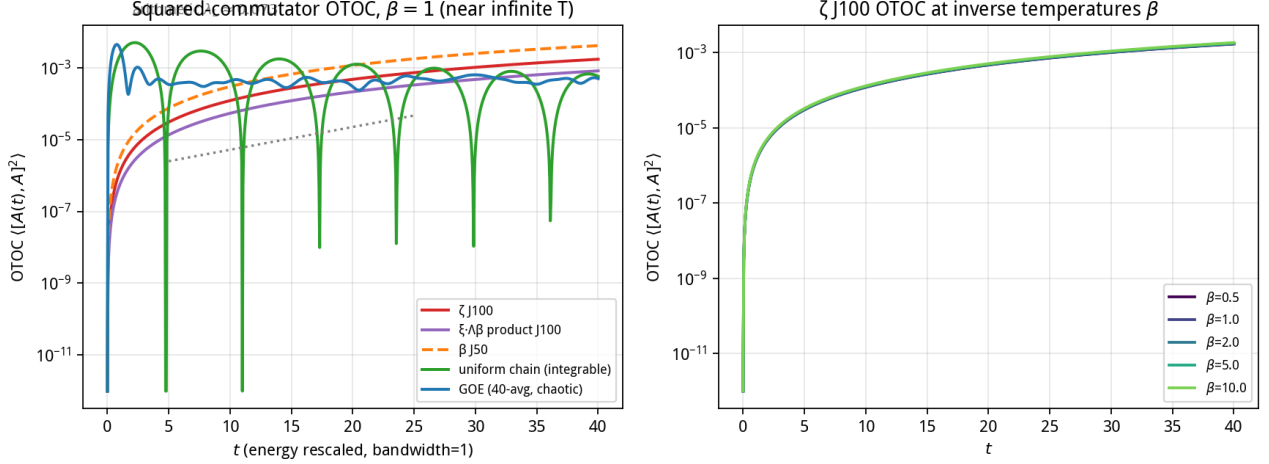
FIG. 8: Out-of-time-order correlator C(t) (log scale). Left: \beta = 1 comparison of five systems: GOE ensemble (40 realizations, instantaneous scrambling), arithmetic chains ( \zeta -J100, \beta -J50, product-J100, all smooth monotonic growth, \lambda_L \approx 0.073 ), uniform chain (periodic revivals, integrable). Right: \zeta -J100 at five inverse temperatures \beta = 0.5, 1, 2, 5, 10 ; the curves overlap, showing \lambda_L is temperature-independent.
