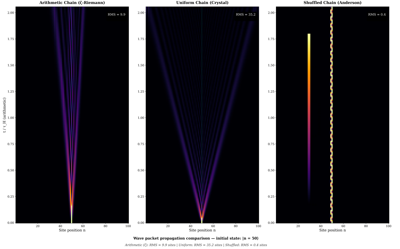
FIG. 4: Experiment 2 (Supplementary). Spatiotemporal evolution |\langle n|\psi(t)\rangle|^2 of a wave packet initialized at the chain center |n=50\rangle for three chains sharing identical coefficient distributions. Left: arithmetic \zeta -Jacobi chain — restricted spreading with RMS displacement \approx 10 , neither ballistic nor fully localized (“pseudo-Anderson” behavior). Center: uniform crystal chain — ballistic light-cone spreading, RMS \approx 35 . Right: shuffled Anderson chain — complete localization, RMS \approx 0.4 ; the wave packet is frozen at the initial site.
