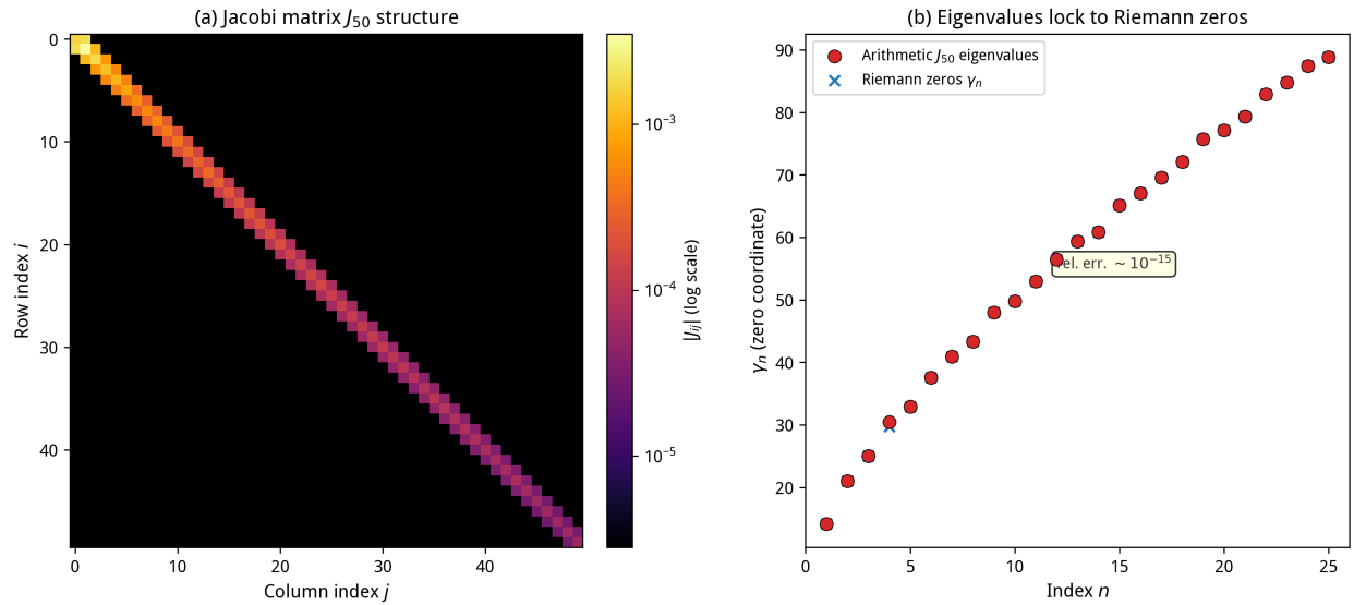
FIG. 1: The arithmetic Hamiltonian at a glance. (a) Log-scale heatmap of the 50 \times 50 Jacobi matrix J_{50} constructed from the Riemann \xi -function: diagonal entries \alpha_n (on-site energies) and off-diagonal entries b_n (hopping amplitudes) are fully determined by 230-digit-precision moments of \xi(s) with zero free parameters . (b) The first 25 eigenvalues of J_{50} (converted to zero coordinates \gamma_n = 1/\sqrt{\lambda_n} ) lock onto the Riemann zeros with relative error \sim 10^{-15} .
