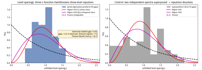
FIG. 2: Experiment 1. Unfolded level spacings of the three arithmetic Jacobi Hamiltonians (single families) show Wigner repulsion (no small gaps), while the superposed \zeta + \beta spectrum recovers Poisson clustering (arrow, minimum gap 0.044).
