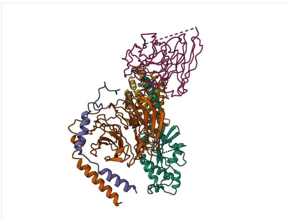
Figure 2: The experimentally characterized MOR–ZH853–Gi–scFv16 cryo-EM complex (Mol* render): \mu -opioid receptor 7TM bundle (gold), G \alpha i (orange), G \beta (teal), G \gamma (purple), and scFv16 (magenta), with ZH853 (green sticks) in the orthosteric pocket.
