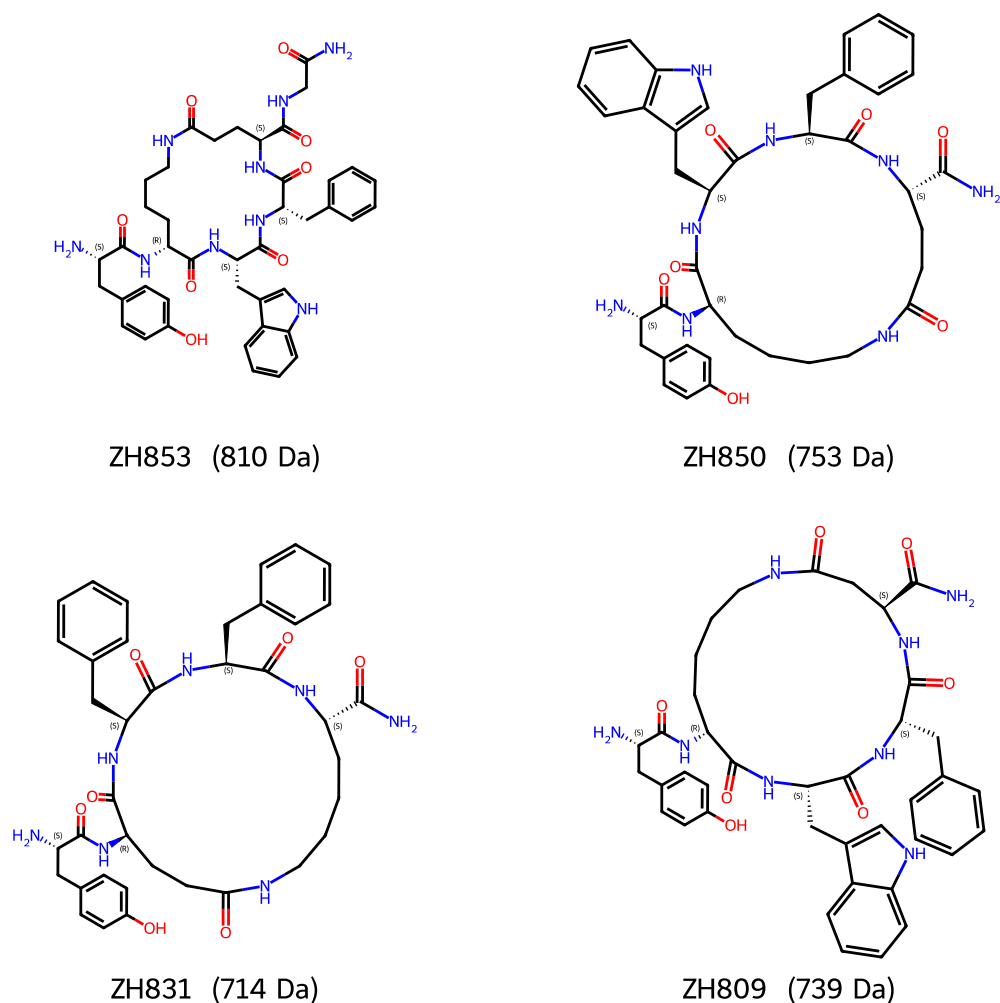
Figure 2: ZH853 and the three FEP analogs (ZH850/831/809), drawn as scaffold-aligned 2D structures with standard atom coloring and CIP stereo descriptors. All are Tyr-cyclo[...]-NH 2 endomorphin-1 macrocycles differing by single-residue substitutions (Trp \leftrightarrow Phe, Glu \leftrightarrow Asp ring size, \pm Gly cap).
