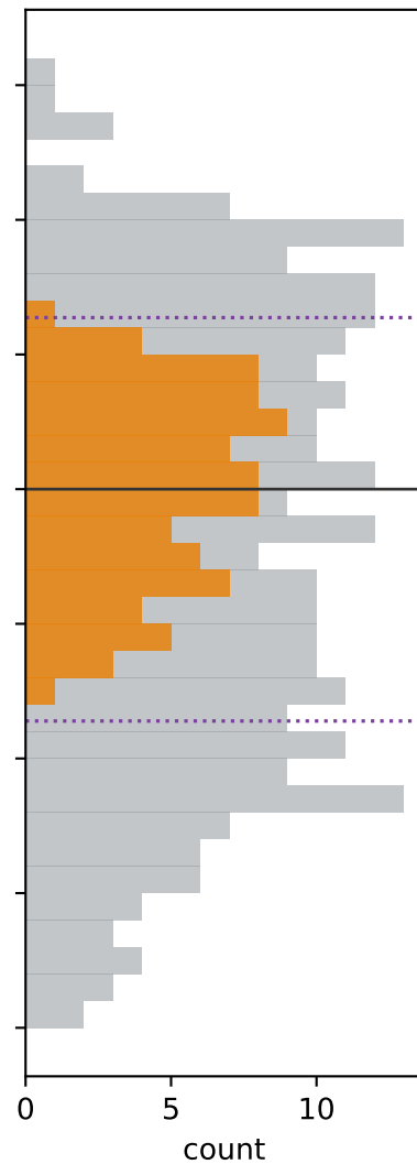
z-distribution
