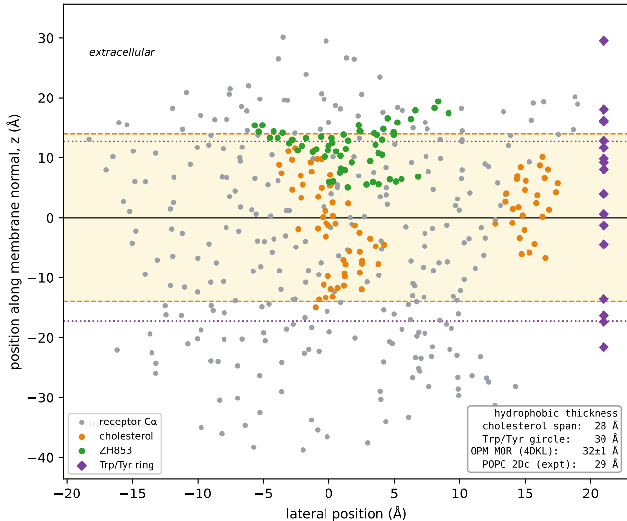
Membrane placement: cholesterol vs aromatic girdle
