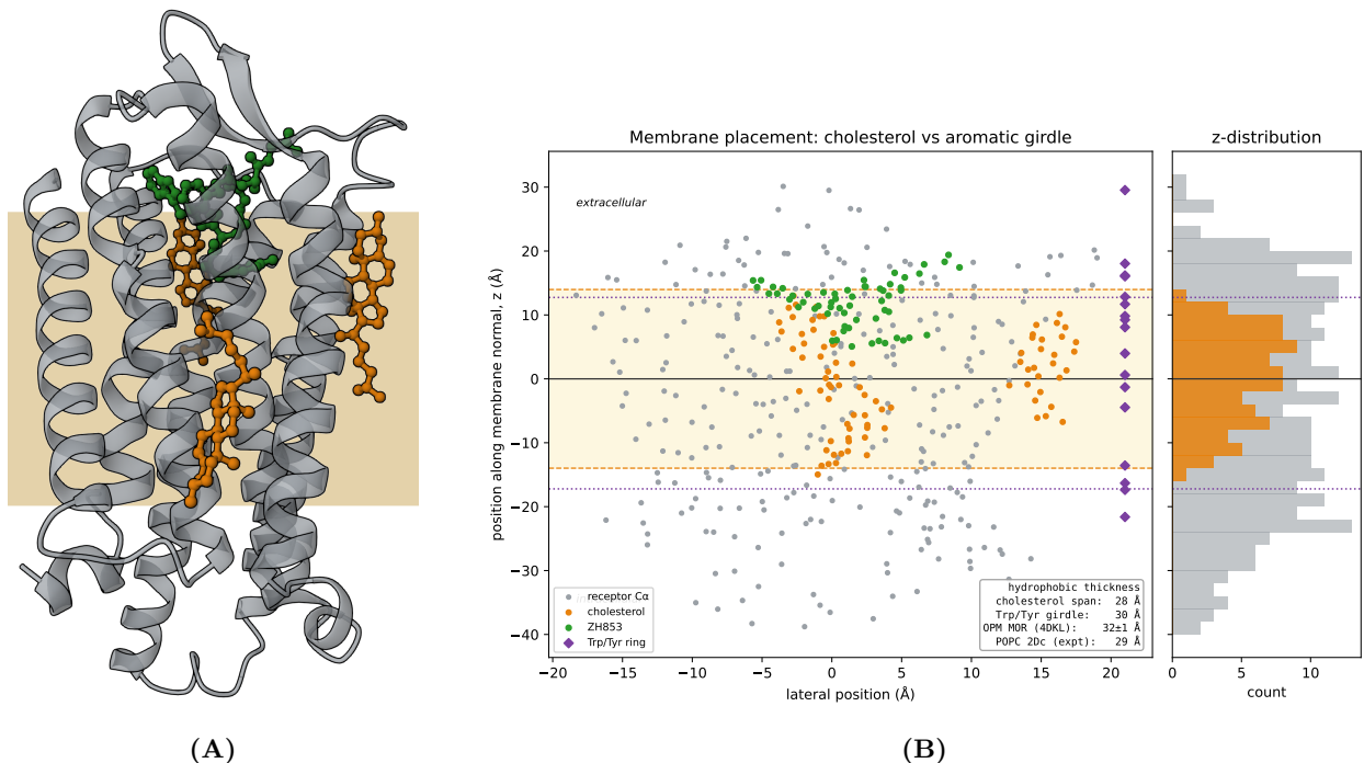
Figure 2: Membrane placement and thickness validation. (A) Side view (Mol* render) of the oriented \mu -opioid receptor (grey cartoon) with the 3 modeled cholesterol (84 atoms; orange, ball-and-stick) and ZH853 (green). The tan band is the inferred hydrophobic core (§3.7), drawn behind the receptor: the transmembrane helices span it and the cholesterol sit within it, while the intracellular loops fall below and ZH853 sits at the extracellular boundary. (B) Cross-check along the membrane normal z : receptor C \alpha (grey), cholesterol (orange), ZH853 (green), and the Trp/Tyr aromatic girdle (purple diamonds; interfaces dotted). The aromatic girdle ( \sim 30 Å) and the cholesterol span ( \sim 28 Å, dashed) bracket the OPM hydrophobic thickness for MOR ( 32 \pm 1 Å) and the experimental POPC hydrocarbon core ( 2D_c = 28.8 Å); ZH853 localizes to the extracellular leaflet. The inferred core is thus physically reasonable; production builds to the OPM \sim 32 Å slab (inset).
