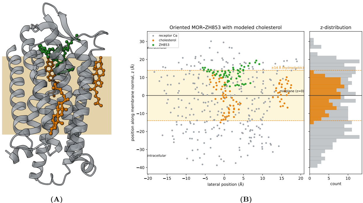
Figure 2: Cryo-EM-anchored membrane placement. (A) Side view (Mol* render) of the oriented \mu -opioid receptor (grey cartoon) with the 3 modeled cholesterol (84 atoms; orange, ball-and-stick) and ZH853 (green). The tan band is the inferred bilayer — the cholesterol-defined midplane and hydrophobic thickness (§3.7) — drawn behind the receptor as a placement sanity check: the transmembrane helices span it and the cholesterol sit within it, while the intracellular loops fall below and ZH853 sits at the extracellular boundary. (B) Determination: distribution along the membrane normal z of cholesterol atoms (orange) and receptor C\alpha (grey). The cholesterol mean fixes the midplane ( z = 0 , solid line) and their span the hydrophobic thickness ( \pm 14 Å, dashed band); ZH853 (green) localizes to the extracellular leaflet. Centring on the cholesterol rather than the C\alpha centroid places the bilayer correctly despite the receptor's z -asymmetry.
