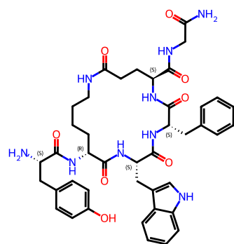
ZH853 (810 Da)
