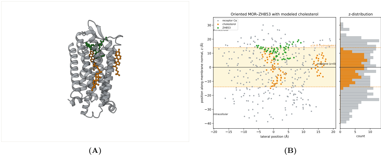
Figure 2: Cryo-EM-anchored membrane placement. (A) Side view (Mol* render) of the oriented \mu -opioid receptor (grey cartoon) with the 84 cholesterols modeled in the density (orange, ball-and-stick) and ZH853 (green). The cholesterols mark the lipid bilayer band directly: the transmembrane helices span it, the intracellular loops hang below, and ZH853 sits at the extracellular boundary; the midplane and thickness this defines are quantified in (B). (B) Determination: distribution along the membrane normal z of cholesterol atoms (orange) and receptor C \alpha (grey). The cholesterol mean fixes the midplane ( z = 0 , solid line) and their span the hydrophobic thickness ( \pm 14\text{ \AA} , dashed band); ZH853 (green) localizes to the extracellular leaflet. Centring on the cholesterols rather than the C \alpha centroid places the bilayer correctly despite the receptor’s z -asymmetry.
