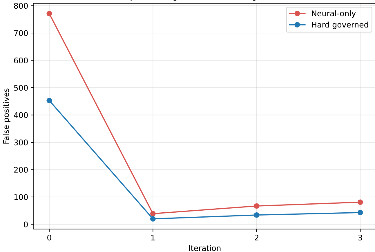
False accepted merges over hard-negative iterations
