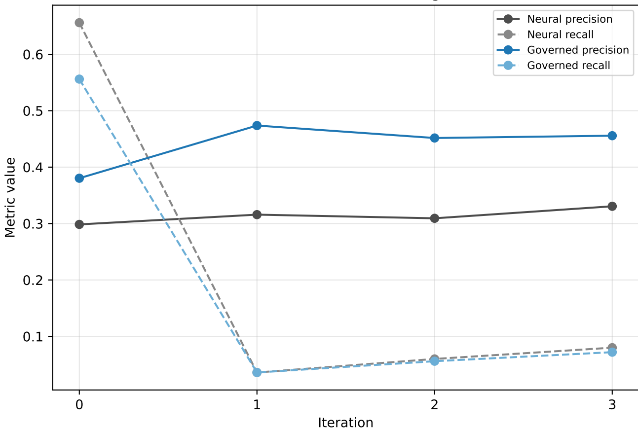
Precision/recall trade-off over hard-negative iterations
