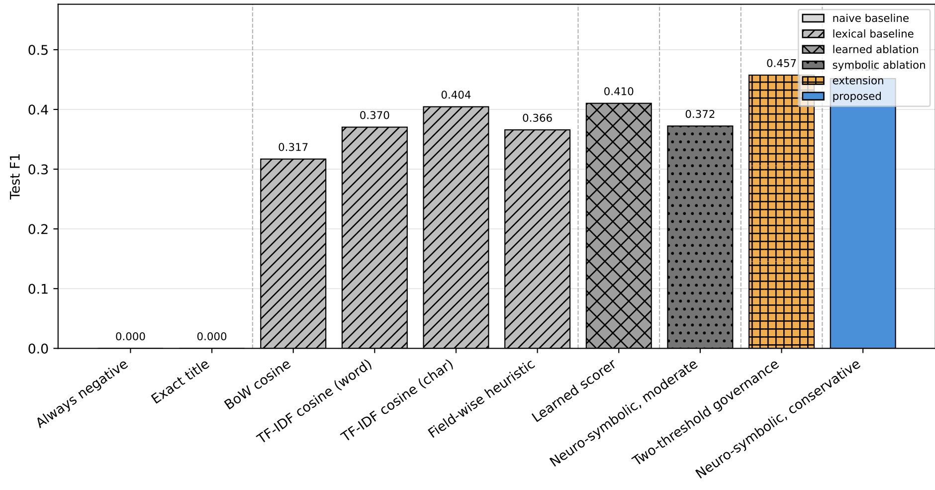
Main comparison: test F1 after validation-based selection
