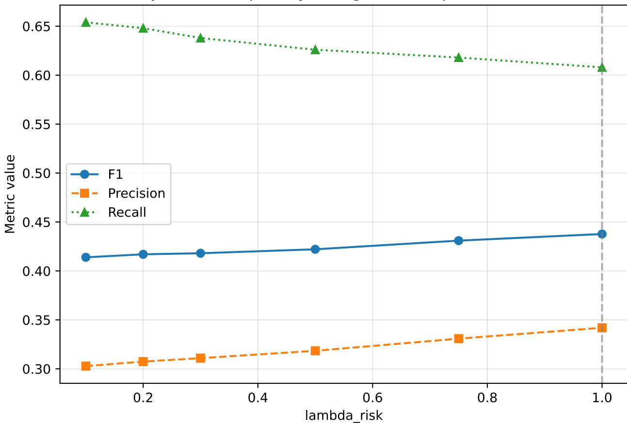
Effect of symbolic risk penalty strength on test performance ( \tau=0.66 )
