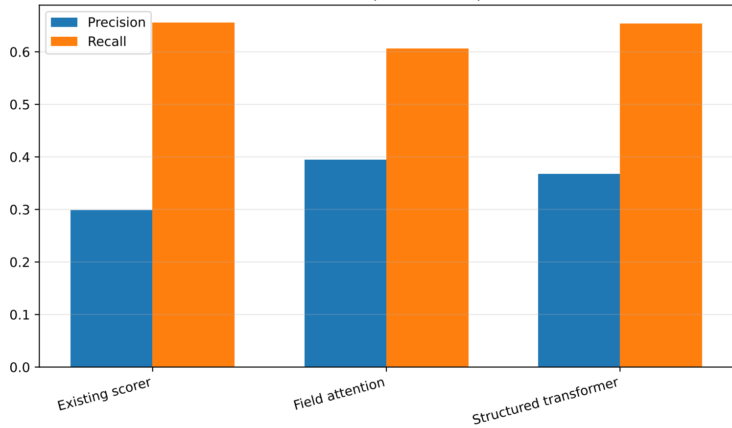
Structured neural scorer comparison: test precision and recall
