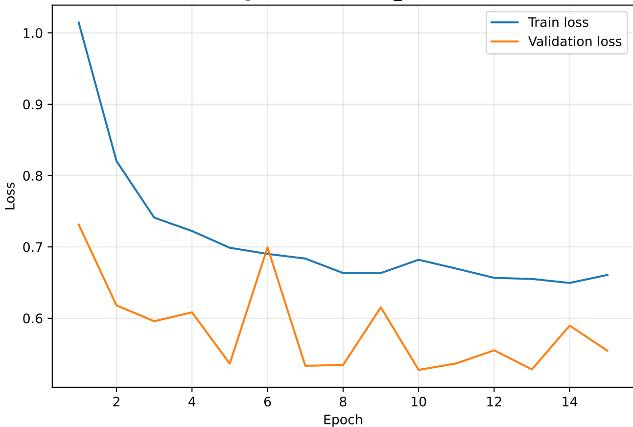
Training curve: structured_transformer
