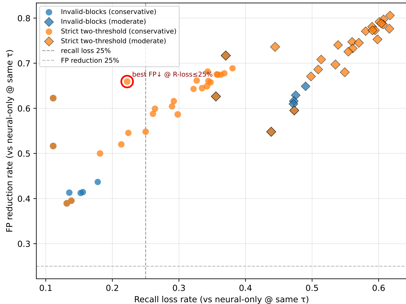
Governance trade-off: FP reduction vs recall loss (test)
