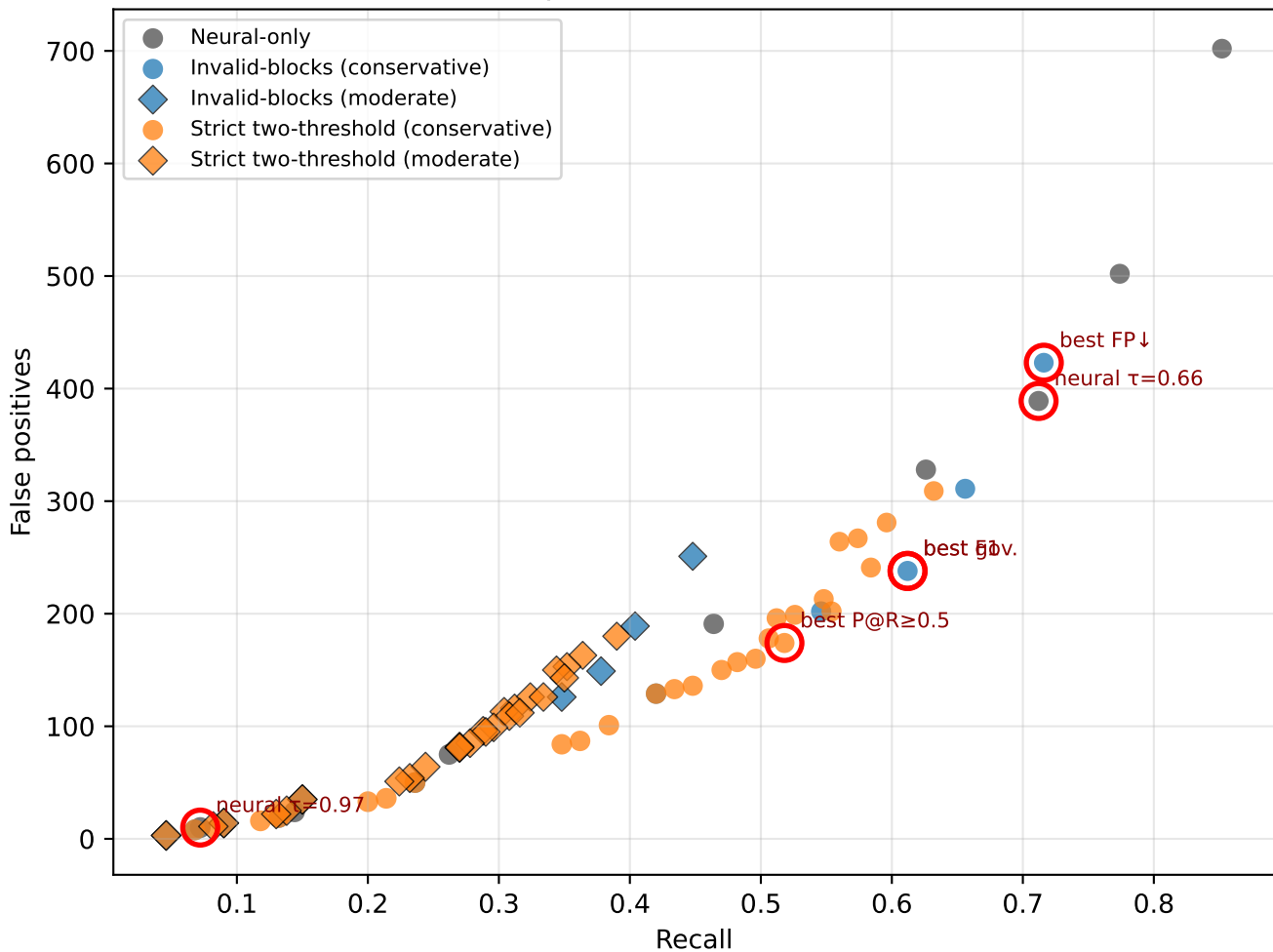
False positives vs recall (valid)
