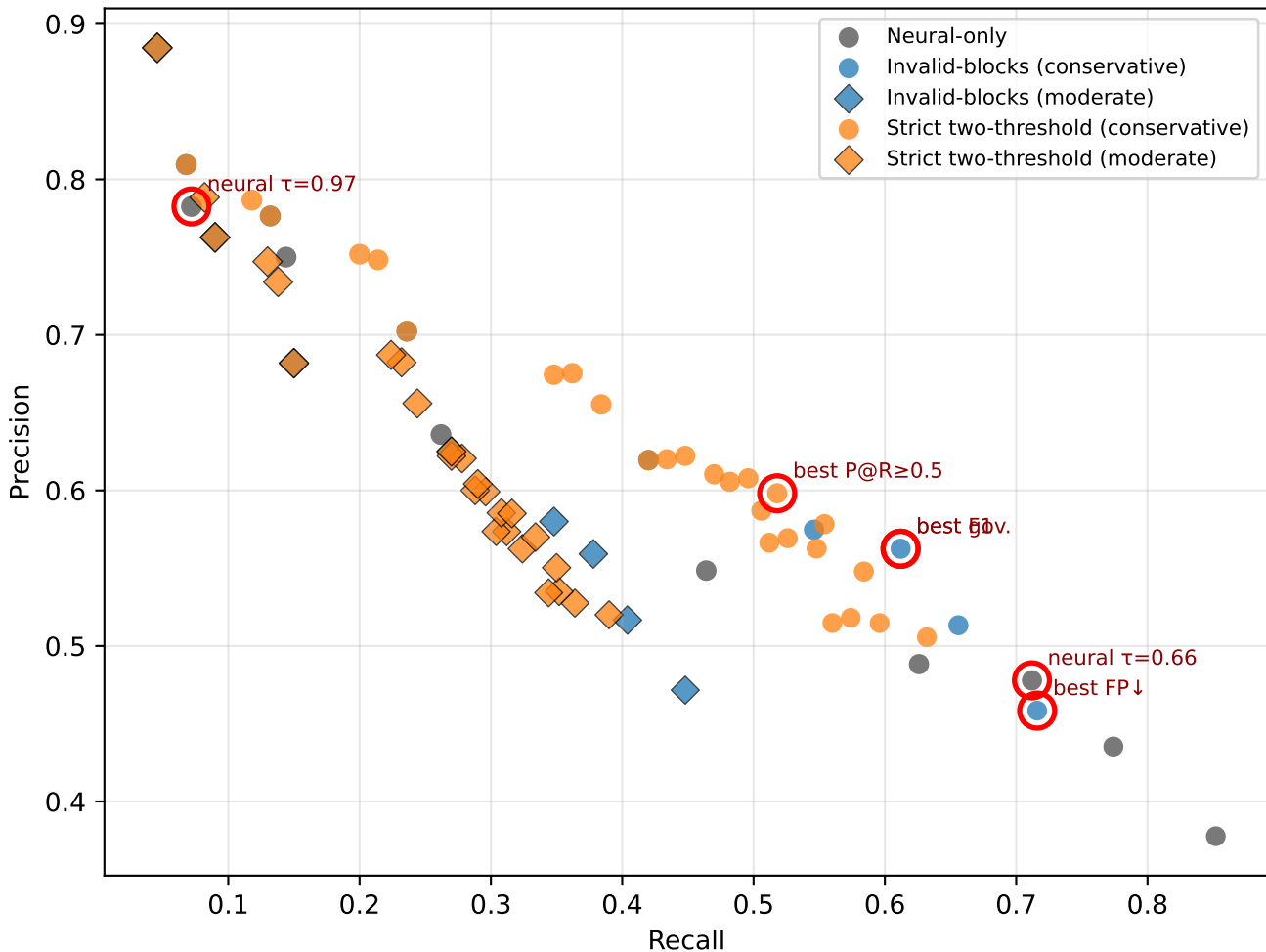
Precision-Recall trade-off (valid)
