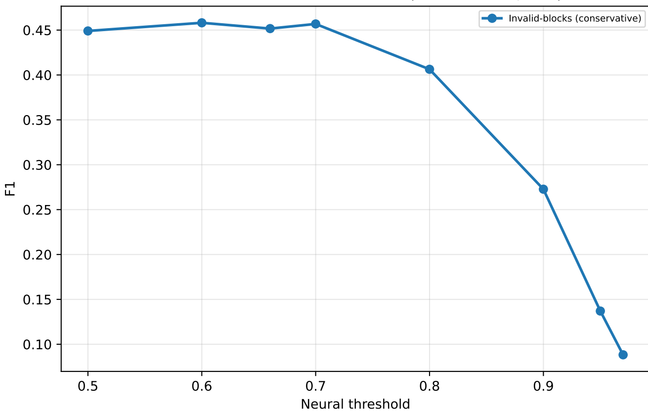
F1 vs threshold — invalid-blocks (conservative, test)
