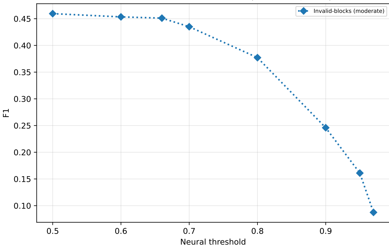
F1 vs threshold — invalid-blocks (moderate, valid)
