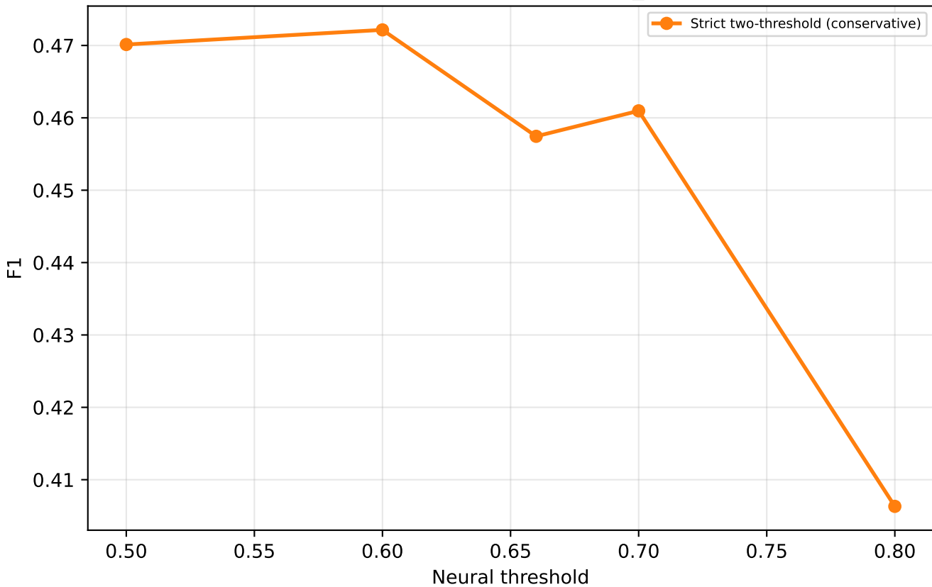
F1 vs threshold — strict conservative \tau_{\text{high}}=0.80 (test)
