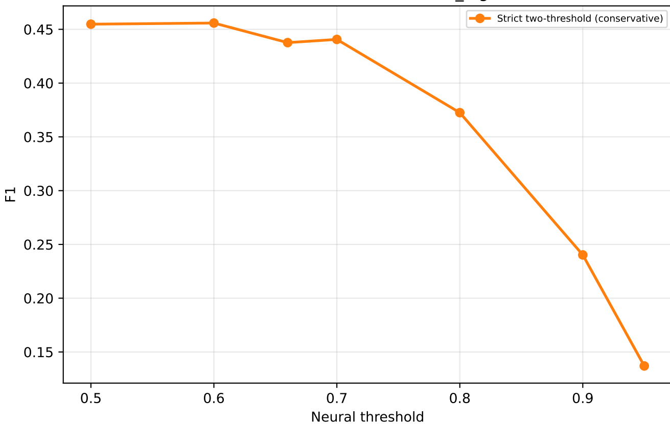
F1 vs threshold — strict conservative \tau_{\text{high}}=0.95 (test)
