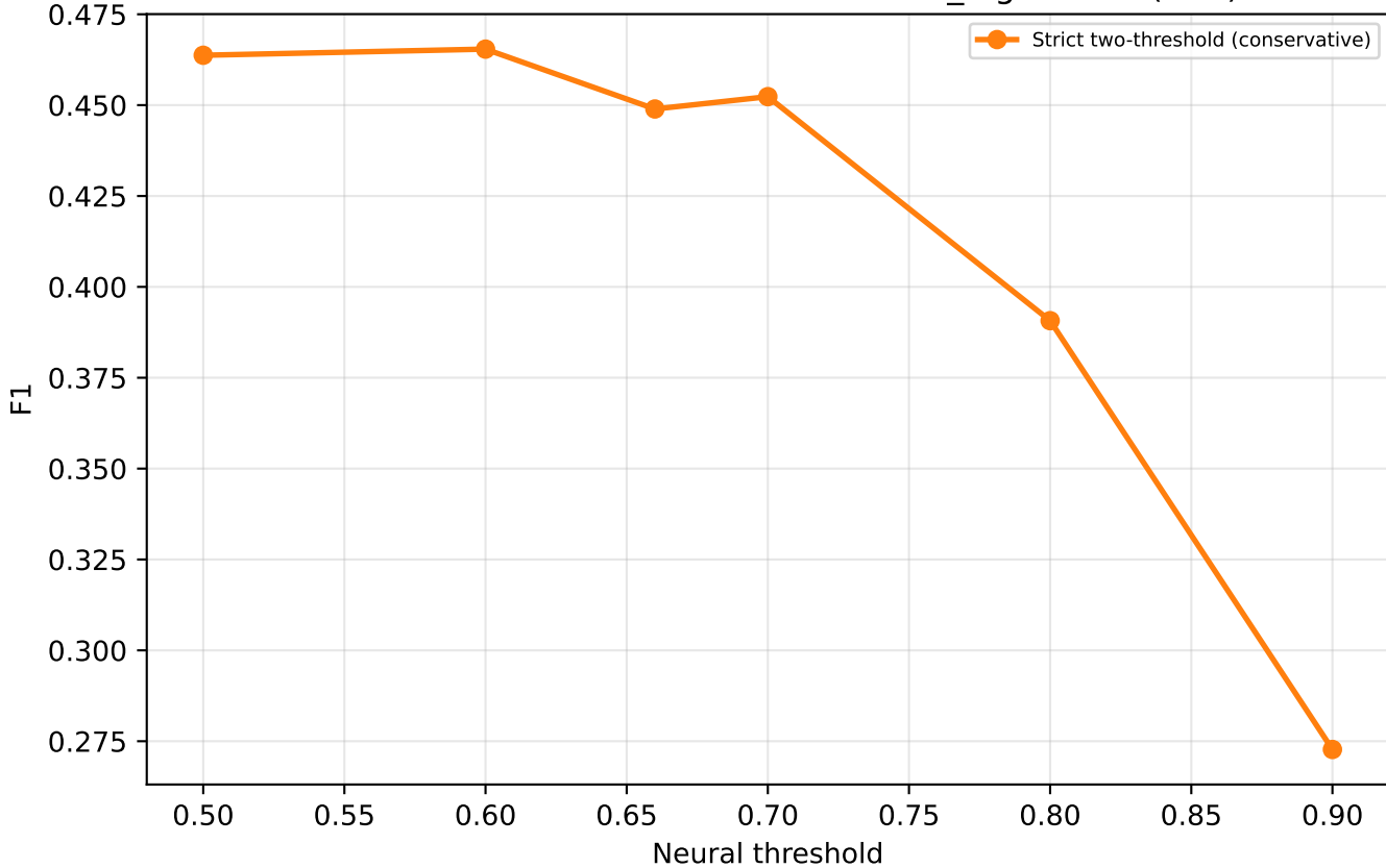
F1 vs threshold — strict conservative \tau_{\text{high}}=0.90 (test)
