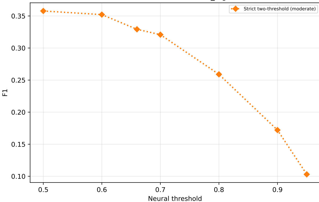
F1 vs threshold — strict moderate \tau_{\text{high}}=0.95 (test)
