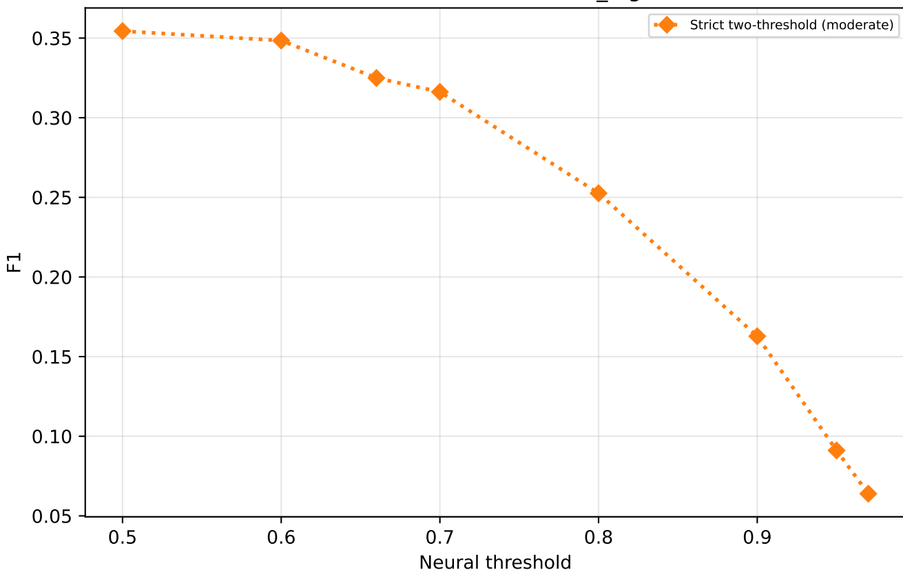
F1 vs threshold — strict moderate \tau_{\text{high}}=0.97 (test)
