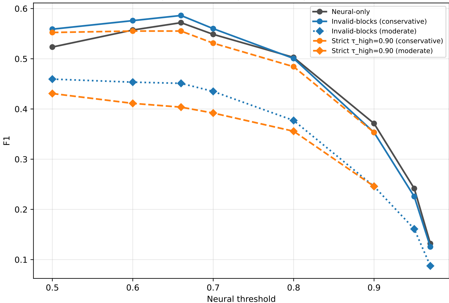
F1 by method (compact summary, valid)
