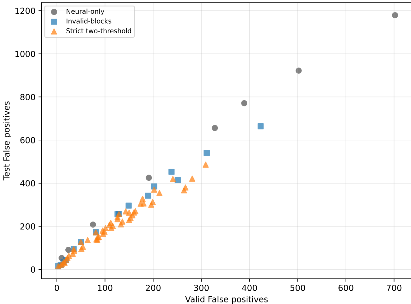
Valid vs test false positives
