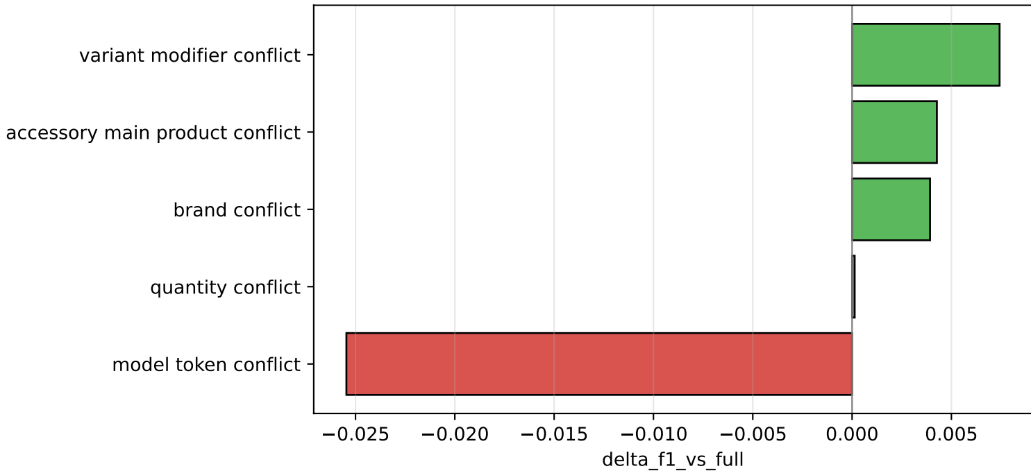
Leave-one-out ablation: delta F1 vs full governance (valid)
